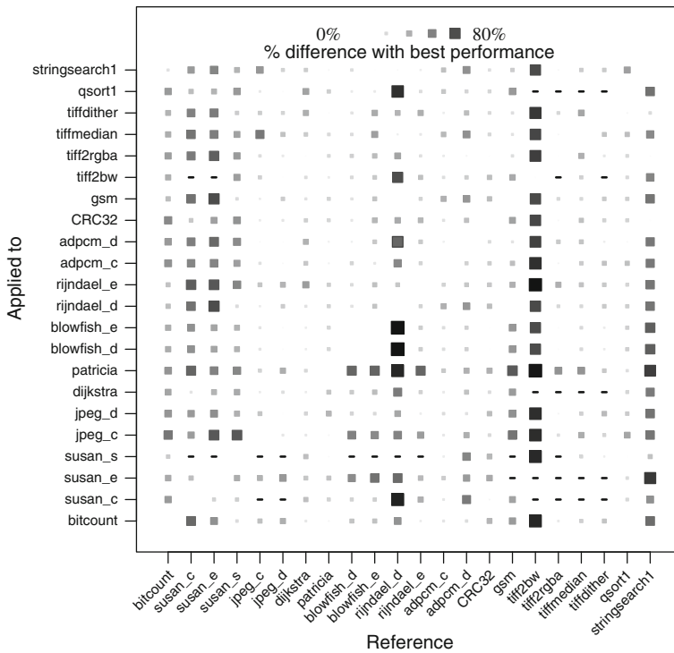
Fig. 8 Percentage difference between speedup achievable after iterative compilation for “applied to” program and speedup obtained when applying best optimization from “reference” program to “applied to” program on AMD. “—” means that best optimization was not found for this program
