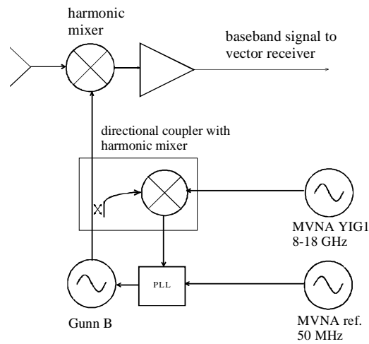
Figure 6. Heterodyne receiver for 300–1000 GHz (ABmm ESA-2).
