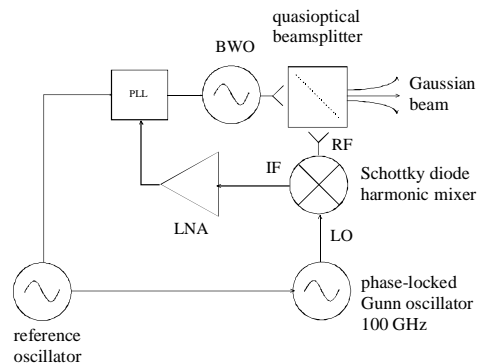
Figure 5. Phase-locked BWO source for 300-1000 GHz (MilliLab).
