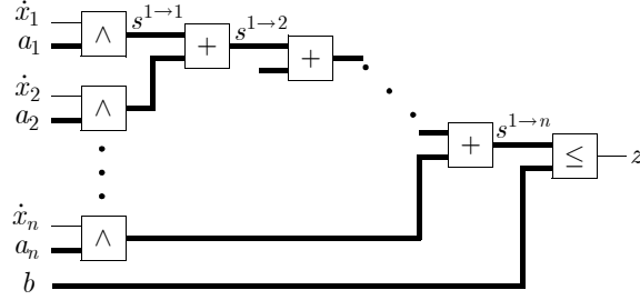
Figure 1: Circuit representation of (4). Single- and multi-bit signals are denoted by thin and bold lines, respectively.
