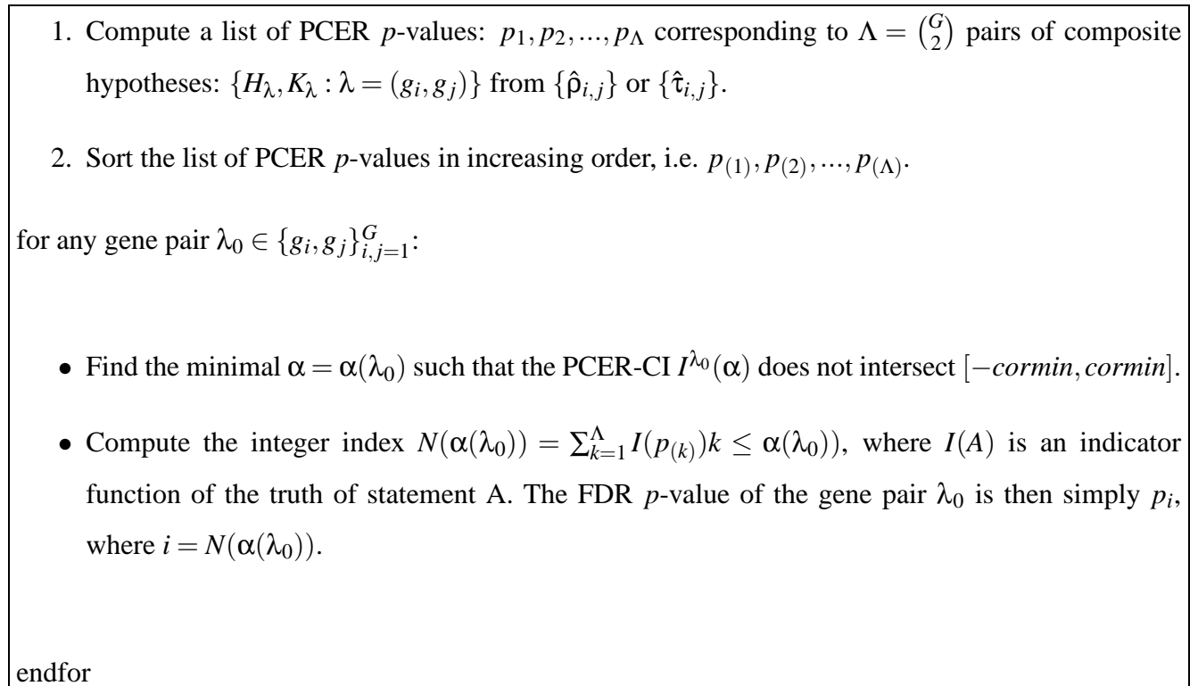
Figure 2: Inverse screening procedure allows the FDR p -value of a gene pair's ( \lambda_0 ) strength of association to be computed.
