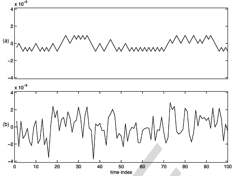
Fig. 3. (a) Noiseless random walk signal with 5 levels. (b) Noisy version of (a) at \text{SNR} = -7.33 dB.
