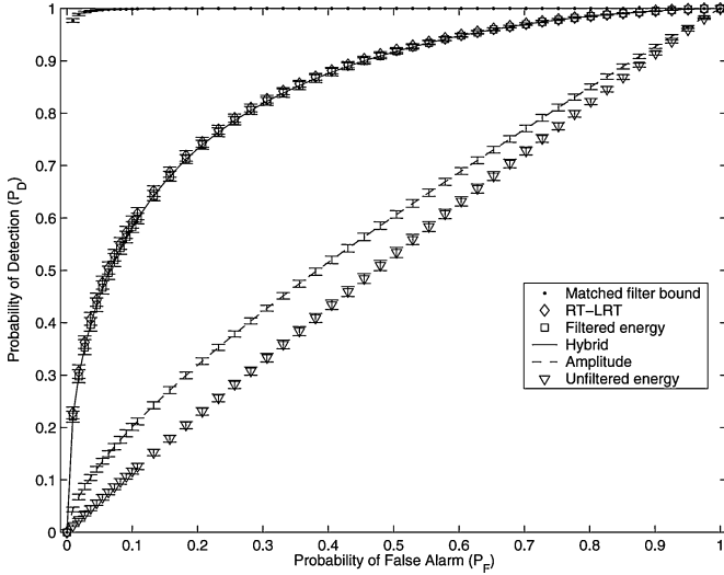
Fig. 4. Simulated ROC curves ( P_D versus P_F ) for the DT random telegraph model with symmetric transition probabilities at \text{SNR} = -34.3 dB, T = 60 s, and \lambda = 0.5 s ^{-1} for the omniscient matched filter, DT random telegraph LRT (RT-LRT), filtered energy, hybrid, amplitude, and unfiltered energy detectors. The RT-LRT is theoretically optimal.
