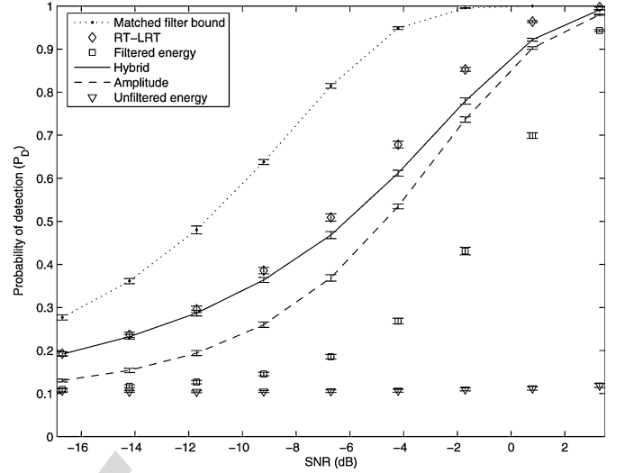
Fig. 8. Simulated power curves for the DT random telegraph model with P_F fixed at 0.1, p = 0.9998 , q = 0.9992 , and T = 150 s. The RT-LRT is theoretically optimal.
