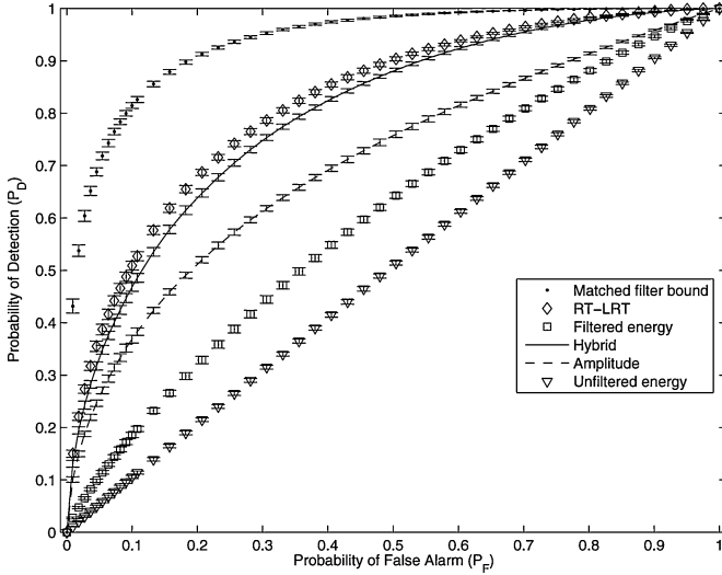
Fig. 7. Simulated ROC curves for the DT random telegraph model with asymmetric transition probabilities ( p = 0.9998 , q = 0.9992 ) at \text{SNR} = -6.71 dB, T = 150 s. The RT-LRT is theoretically optimal.
