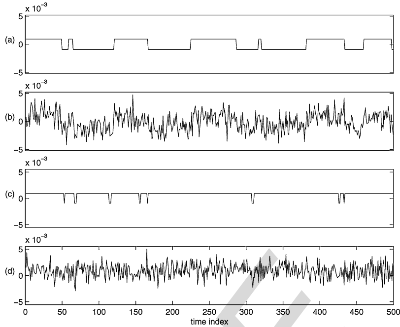
Fig. 2. (a) Noiseless random telegraph signal with symmetric transition probabilities p = q = 0.98 . (b) Noisy version of (a) at \text{SNR} = 7.09 dB. (c) Noiseless random telegraph signal with asymmetric transition probabilities p = 0.98 , q = 0.6 . (d) Noisy version of (c) at \text{SNR} = 13.9 dB.
