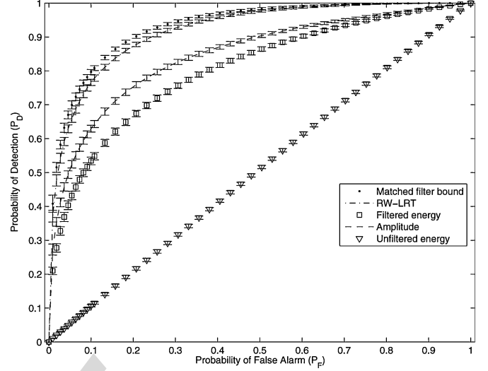
Fig. 11. Simulated ROC curves for the DT asymmetric random walk p_{l,1} = p_{u,1} = 0.45 , p_{l,2} = p_{u,2} = 0.55 at SNR = -2.50 dB, T = 60 s. The RW-LRT is theoretically optimal.
