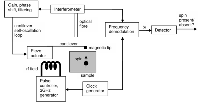
Fig. 1. Schematic of an OSCAR-type MRFM experiment. <AUTHOR: If you prefer, you may submit a figure with larger size font in tiff, ps, eps, Word, Powerpoint, Excel or jpeg format with corrections—ed.>
