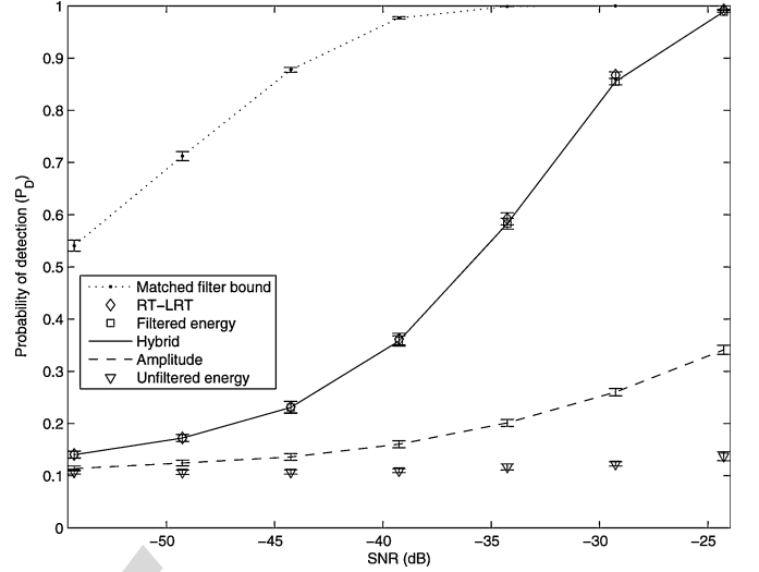
Fig. 5. Simulated power curves ( P_D versus SNR) for the DT random telegraph model with P_F fixed at 0.1 and \lambda = 0.5 s ^{-1} , T = 60 s. The RT-LRT is theoretically optimal.
