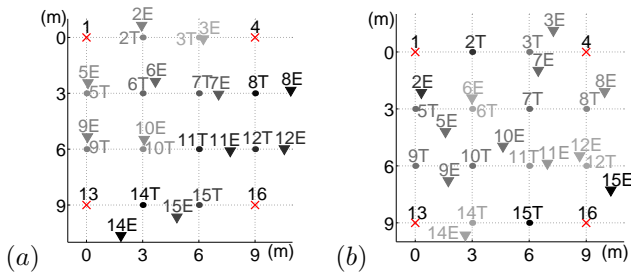
Fig. 7. True (●#T) and estimated (▼#E) location for the (a) parking lot and (b) residential home tests, using 4 reference devices (X#). Higher errors are indicated by darker text.
