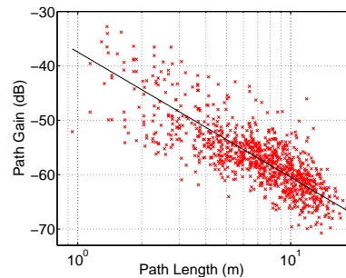
Fig. 4. Measured wideband path gain (x) as a function of path length. Linear fit (-) is with d_0 = 1 m, n_p = 2.3 , and \sigma_{dB} = 3.92 .
