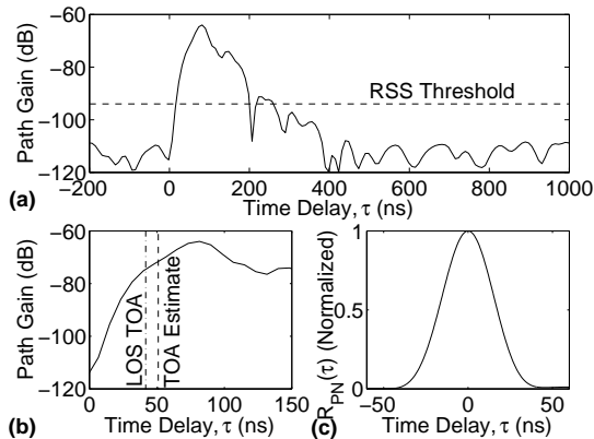
Fig. 3. (a) Measured PDP with TX at 1 and RX at 24 and threshold (- - -) above which received power is integrated to calculate RSS. (b) Leading edge of same PDP showing LOS TOA = d_{1,24}/c (· · · · ·) and estimated TOA (- - -). (c) Autocorrelation of PN signal R_{PN}(\tau) used in template-matching [23].
