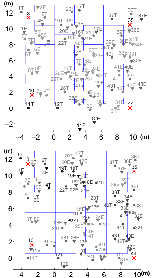
Fig. 6. True ( \bullet\#T ) and estimated ( \blacktriangledown\#E ) location using (a) RSS and (b) TOA data for measured network with 4 reference devices ( X\# ). Higher errors are indicated by darker text.
