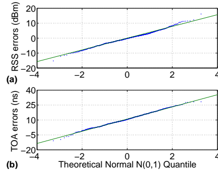
Fig. 5. Q-Q plot of (a) P_{i,j}(\text{dBm}) - \bar{P}_{i,j}(\text{dBm}) for RSS data, and (b) T_{i,j} - d_{i,j}/c for TOA data, compared to a Gaussian quantile.
