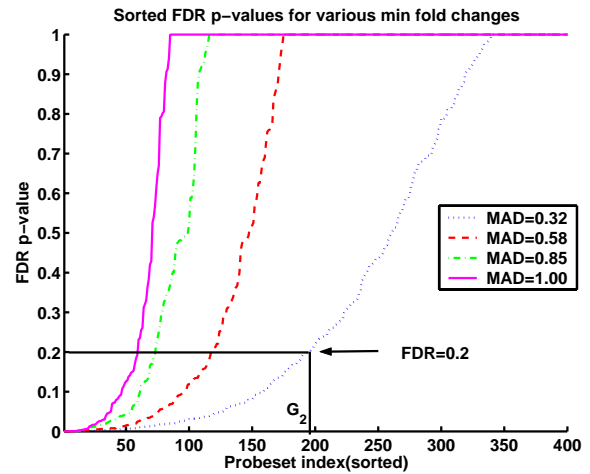
Figure 4. Plots of FDR p-value curves over sorted list of gene indices for 4 values of the minimum acceptable difference (MAD) criterion: f_{\text{cm}} = 0.32, 0.58, 0.85, 1.0 (log base 2) corresponding to wild-type/knockout MAD ratios of 1.25, 1.5, 1.8, and 2.0, respectively. Constraints FDR \leq 0.2 and \text{foldchange} > 0.32 determine a set \mathcal{G}_2 of \mathcal{G}_2 differentially expressed genes by thresholding the corresponding curve as indicated.
