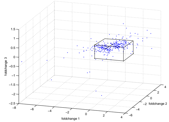
Figure 2. Three dimensional multicriteria space for knock-out and wild-type profiles over 3 time points shown in Fig. 1. The 3 criteria are the differential probe responses at each time point. Shown is a scatter plot of sample means of the differential responses along with a box of edge length 2\text{fcmin} distinguishing biologically significant responses (outside box) from biologically insignificant responses (inside box).
