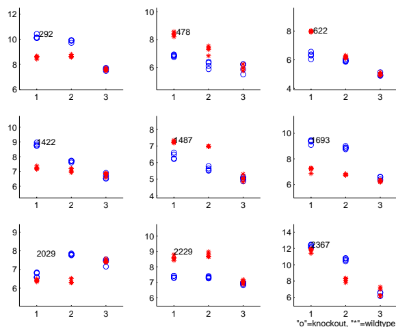
Figure 5. Gene profiles of 9 of the differentially expressed genes discovered using proposed two stage FDR-CI procedure with constraints on level of significance \alpha = 0.2 and minimum foldchange f_{cmin} = 1.0 . Knockout “o” and Wildtype “*” are as indicated.
