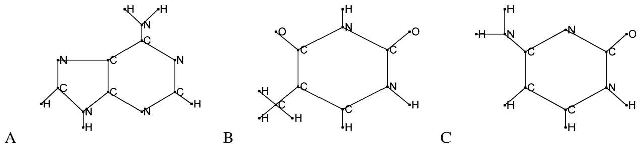
Fig. 5. Chemical graphs derived from the familiar molecules from DNA: adenine (A), thymine (B), and cytosine (C).
