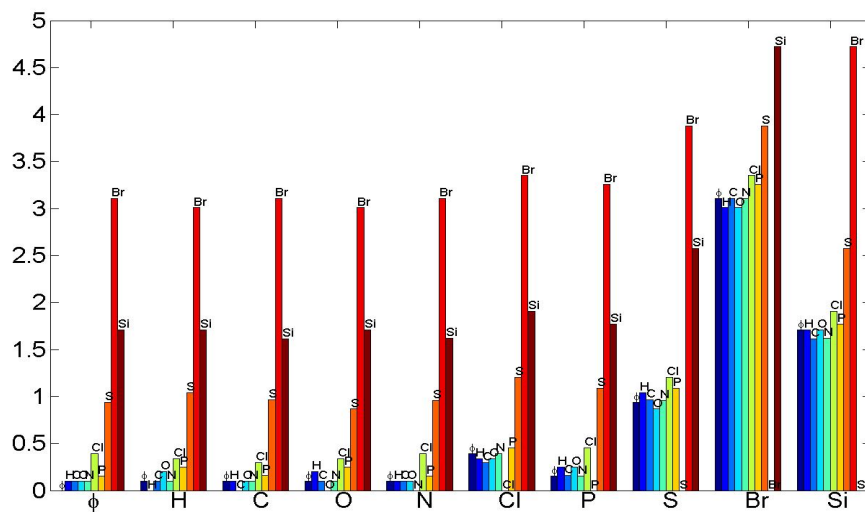
Fig. 6. Optimal edit costs resulting from the convex program in Eq. (21). There is a label associated with each group of bars. Within the group, the edit cost of changing the group label to an individual label corresponds to the height of the bar below that individual label. The optimal edge edit cost c(0, 1) was 0.1.
