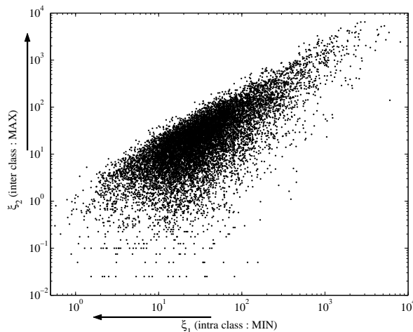
Figure 4: The multicriterion scattergram for the human retina aging experiment. Each point in the scatterplot corresponds to the pair (\xi_1(n), \xi_2(n)) for a particular gene n .
