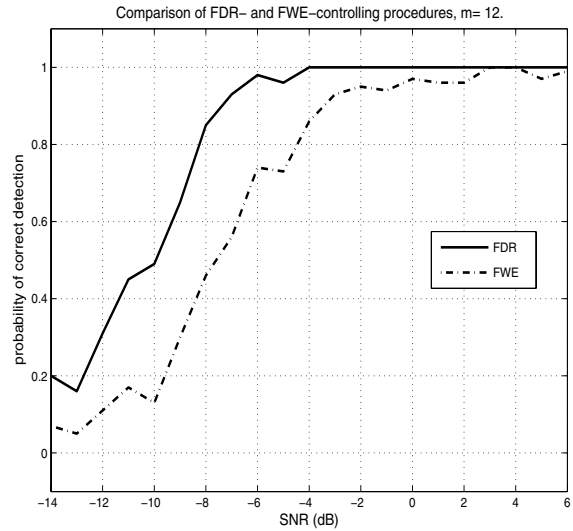
Fig. 1. Probability of correct detection. M = 12 , \text{SNR} = [-14 : 1 : 6] dB, number of frequency bins J = 10 , number of snapshots K = 5 . All sources are apart more than 7^\circ .
