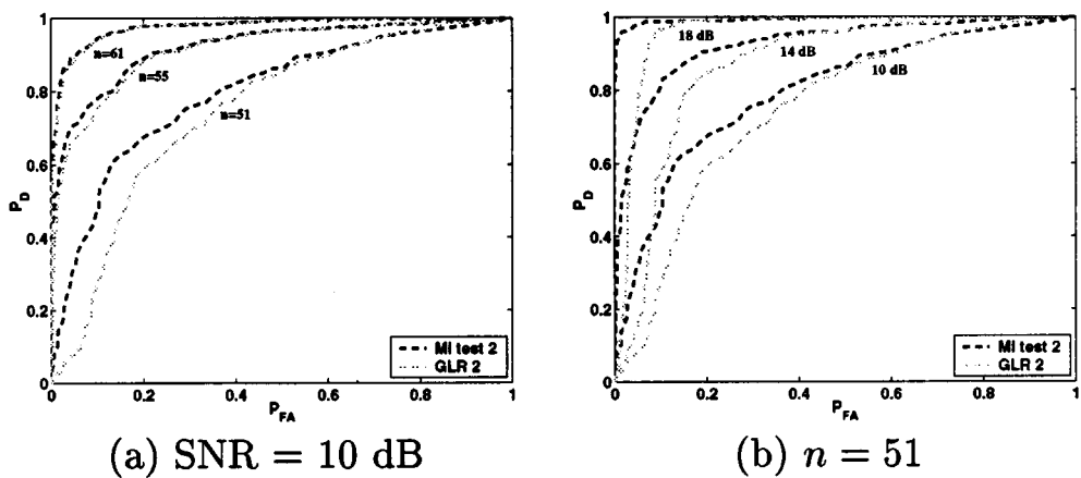
Fig. 4. Comparison of GLR and MI tests for Case 2 by (a) increasing n with fixed SNR and (b) increasing SNR with fixed n ( m_A = 50, m_B = 50 ).
