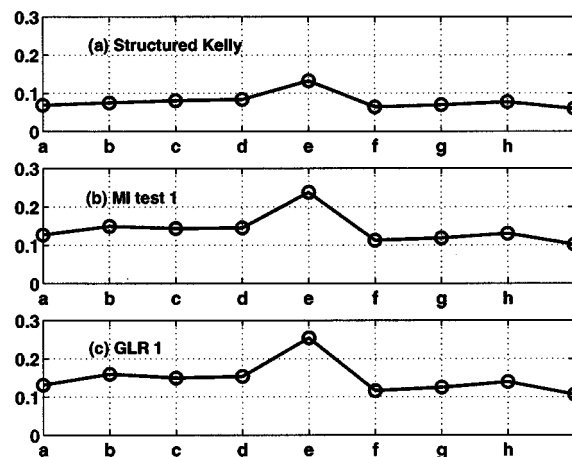
Fig. 9. Peak values obtained for nine different target images in Fig. 7 ( |a| = 0.015, n - 1 = 250 ).
