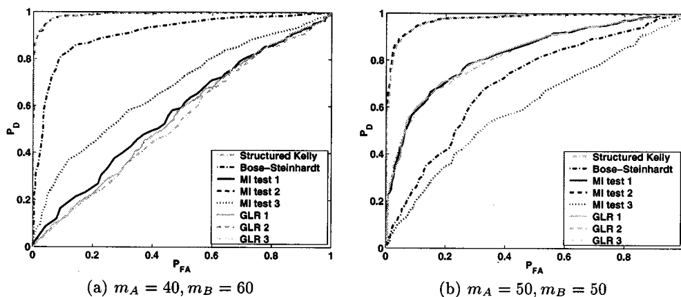
Fig. 2. ROC curves for Case 2 with different ratios of m_A/m_B (SNR = 10 dB, n = 61 ).
