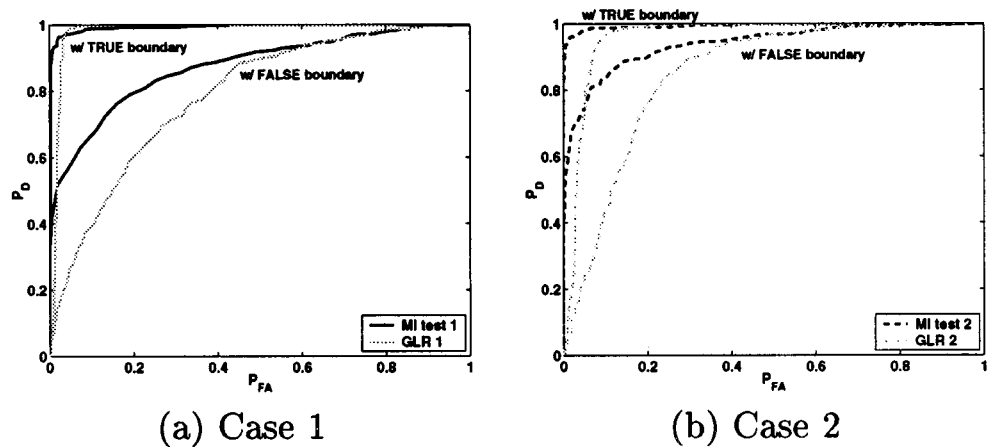
Fig. 5. Comparison of ROC curves using true boundaries and false boundaries (a) moved downward by one pixel and (b) moved upward by one pixel in each snapshot. (True values: (a) m_A = 60, m_B = 40, n = 61 and (b) m_A = 50, m_B = 50, n = 51 ).
