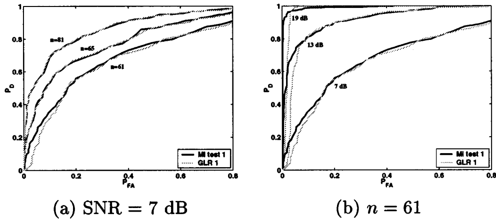
Fig. 3. Comparison of GLR and MI tests for Case 1 by (a) increasing n with fixed SNR and (b) increasing SNR with fixed n ( m_A = 60, m_B = 40 ).
