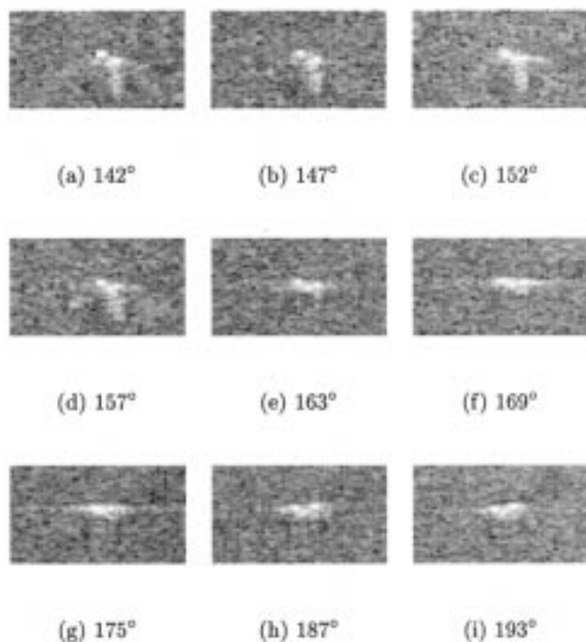
Fig. 7. Magnitude images of SLICY canonical targets at elevation 39° and different azimuth angles. Image in (e) is inserted in Fig. 6.
