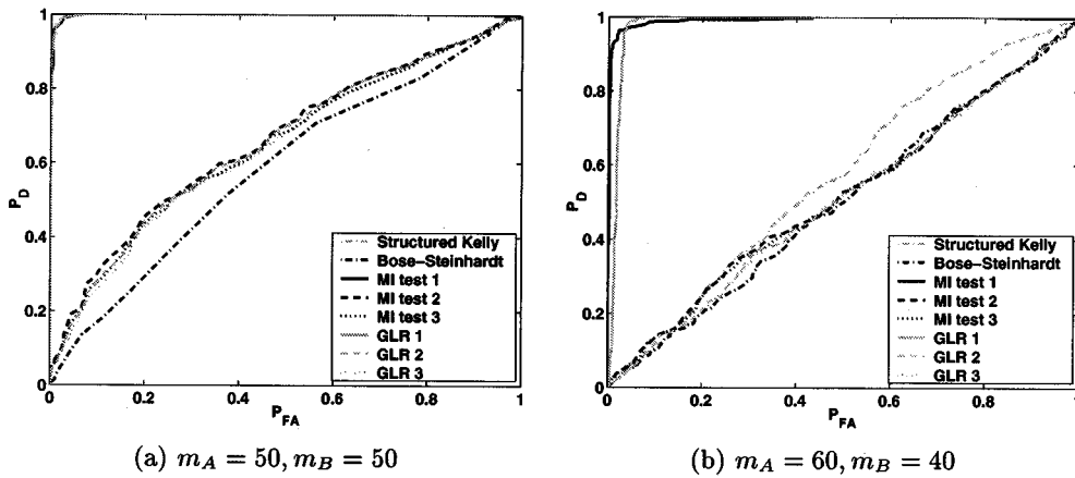
Fig. 1. ROC curves for Case 1 with different ratios of m_A/m_B (SNR = 19 dB, n = 61 ).
