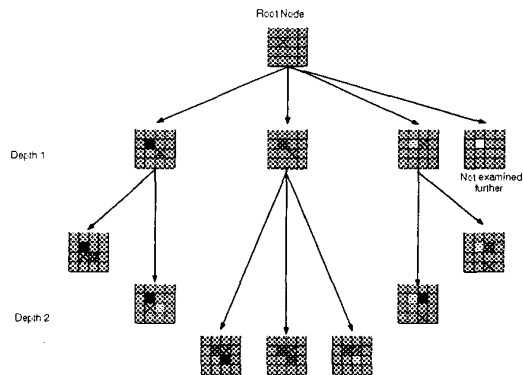
Fig. 1. Part of feature tree data structure.
