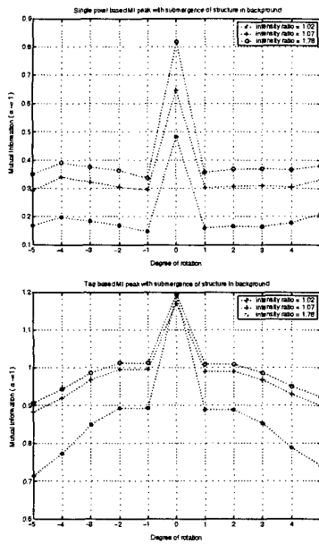
Fig. 5. Upper curves are single pixel based MI trajectories while lower curves are 4 \times 4 tag based MI trajectories for bar images.
