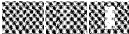
Fig. 4. Bar images with contrast 1.02, 1.07 and 1.78. Background is low variance white Gaussian while bar is uniform intensity.
