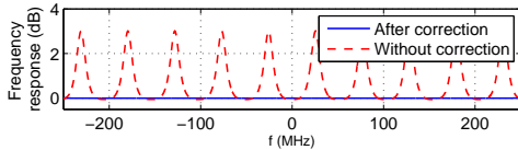
Fig. 4. PR condition. Dot line represents 20 \log_{10} |\sum_l H(f + lf_p)| , and solid line represents 20 \log_{10} |\sum_l T(f + lf_p)| .
