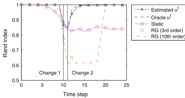
Fig. 11 Comparison of Rand index in two colliding Gaussians experiment. The estimated \alpha^t detects the changes in clusters quickly unlike the RG method
