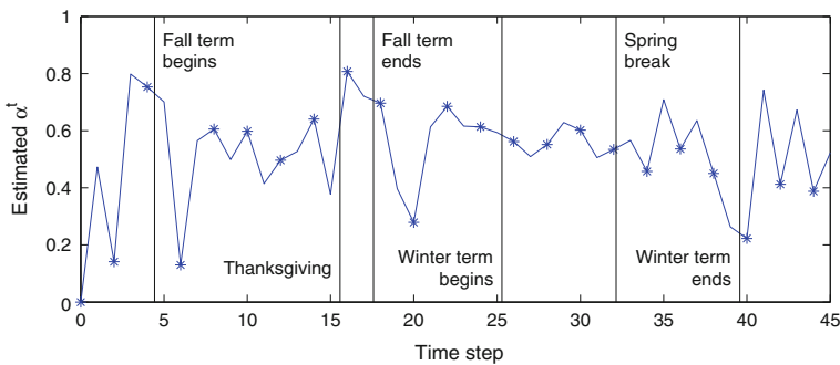
Fig. 18 Estimated \alpha^t over entire MIT Reality Mining data trace. Six important dates are indicated. The sudden drops in the estimated \alpha^t indicate change points in the network
