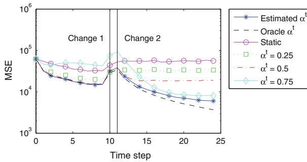
Fig. 10 Comparison of MSE in two colliding Gaussians experiment. The estimated \alpha^t performs best both before and after the change points
