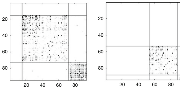
Fig. 19 Cluster structure before (left) and after (right) beginning of winter break in MIT Reality Mining data trace. Darker entries correspond to greater time spent in physical proximity. The empty cluster to the upper left consists of inactive participants during the time step
