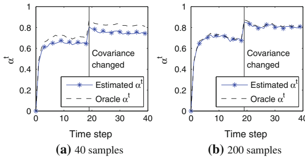
Fig. 8 Comparison of oracle and estimated forgetting factors in well-separated Gaussians experiment. The gap between the estimated and oracle forgetting factors decreases as the sample size increases
