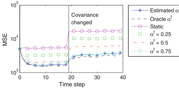
Fig. 7 Comparison of MSE in well-separated Gaussians experiment. The adaptively estimated forgetting factor outperforms the constant forgetting factors and achieves MSE very close to the oracle forgetting factor
