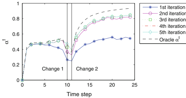
Fig. 12 Comparison of oracle and estimated forgetting factors in two colliding Gaussians experiment. There is no noticeable change after the third iteration
