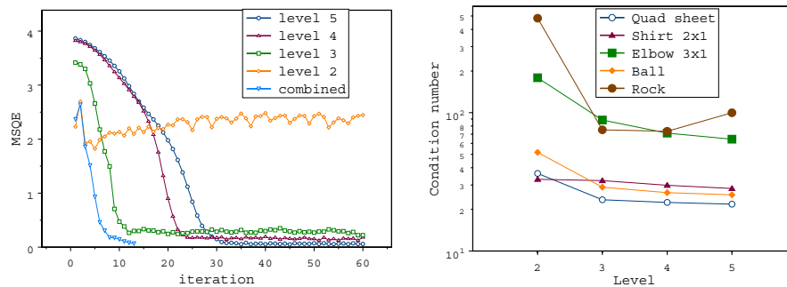
Fig. 1. Left: mean-square error during iterations of template matching procedures at different levels of template resolution. Right: comparison of condition numbers of H^t H matrices at different levels of resolution. For quad patterns the condition number stays relatively low on all the levels, while for natural patterns it is less controlled.
