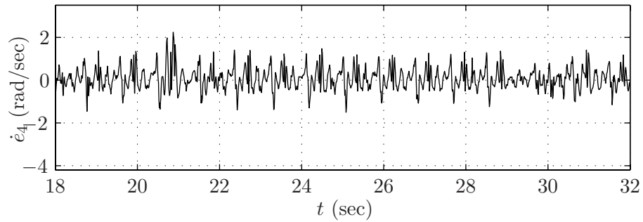
(d) e_4 = \dot{q}_4 - (\partial h_{d,4}/\partial \hat{\theta})\dot{\hat{\theta}} versus time.
