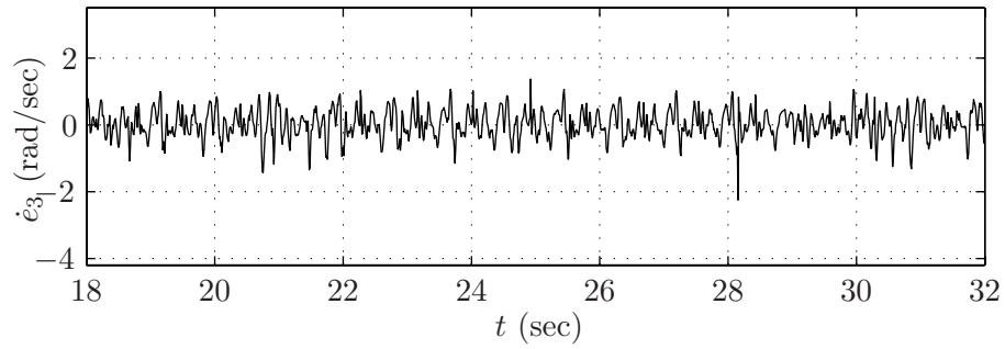
(b) e_3 = \dot{q}_3 - (\partial h_{d,3}/\partial \hat{\theta})\dot{\hat{\theta}} versus time.
