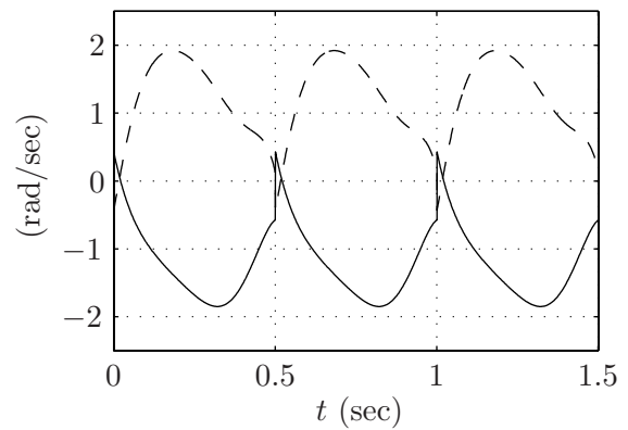
(d) \dot{q}_1 (solid) and \dot{q}_2 (dashed) versus time.
