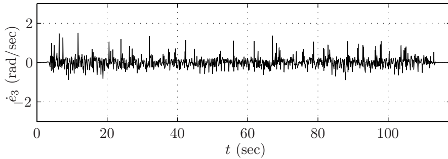
(b) \dot{e}_3 = \dot{q}_3 - (\partial h_{d,3}/\partial \hat{\theta})\hat{\theta} versus time.
