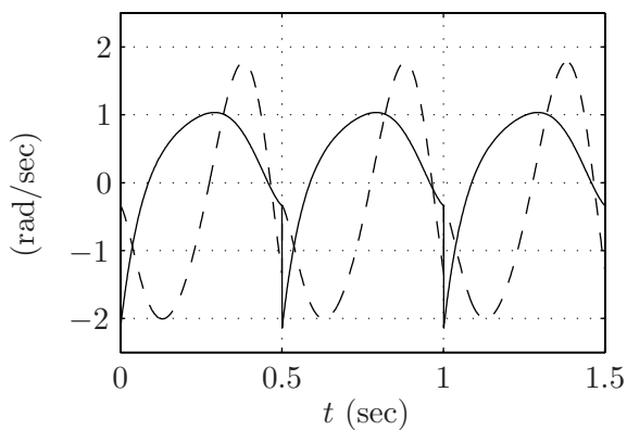
(e) \dot{q}_3 (solid) and \dot{q}_4 (dashed) versus time.
