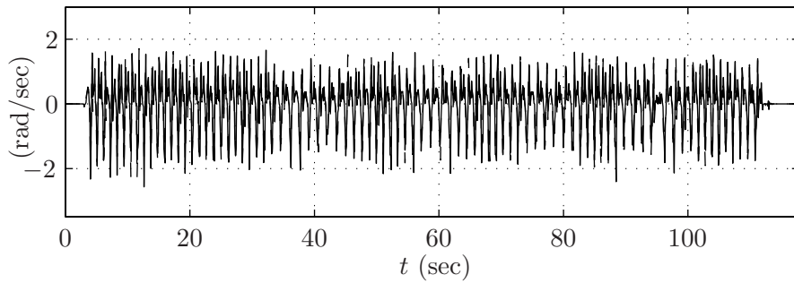
(c) \dot{q}_4 (solid) and (\partial h_{d,4}/\partial \hat{\theta})\hat{\theta} (dashed) versus time.
