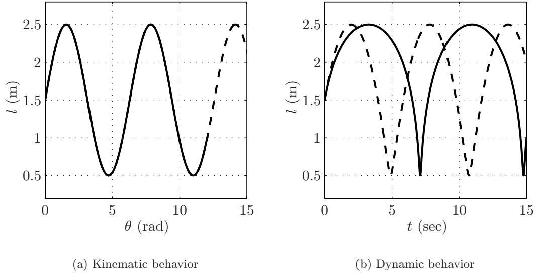
Figure 3.3: Kinematic and dynamic behaviors of the horizontal pendulum. The dashed lines correspond to the constraint l = \sin(\theta) + 1.5 imposed via a physical constraint, whereas the solid corresponds to the same constraint imposed via a virtual constraint.
