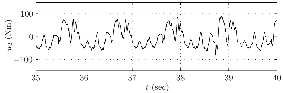
(b) u_2 versus time.
