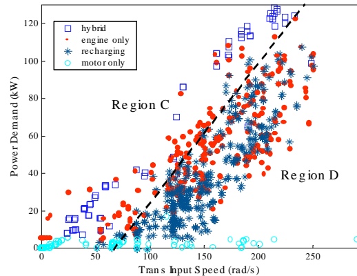
Figure 8: Operating points of DP optimization over UDDSHDV cycle without regenerative braking
