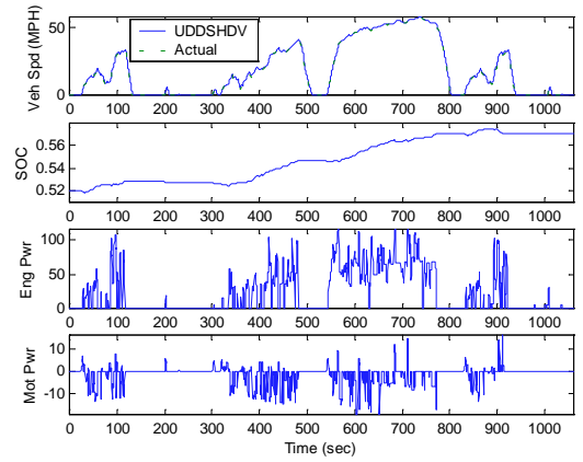
Figure 7: Simulation results of UDDSHDV cycle without regenerative braking
