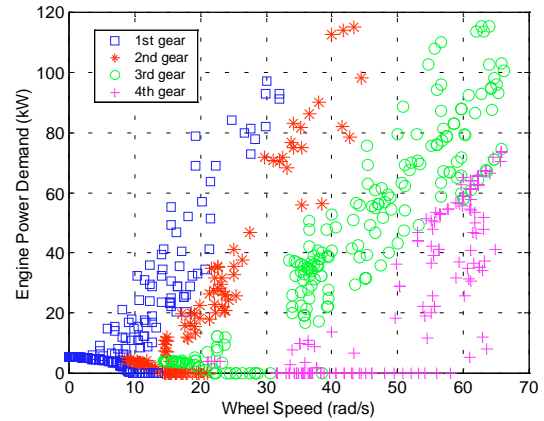
Figure 5: Gear operating points of DP optimization
