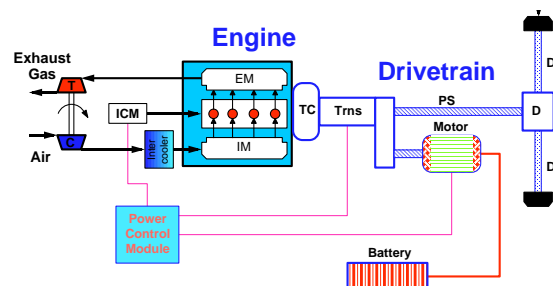
Figure 1: Schematic diagram of the hybrid electric truck
