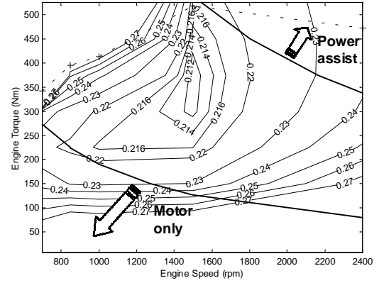
Figure 3: Power Split Control strategy
