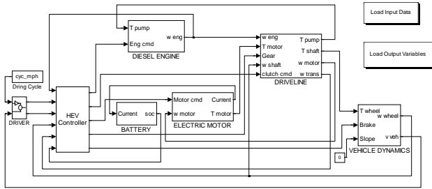
Figure 2: Hybrid-electric vehicle simulation in SIMULINK
