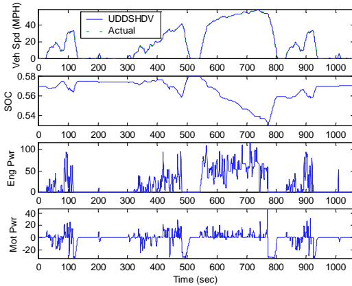
Figure 4: Simulation result of UDDSHDV cycle. The engine and motor power are given in kW
