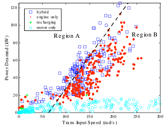
Figure 6: Operating points of DP optimization over UDDSHDV cycle
