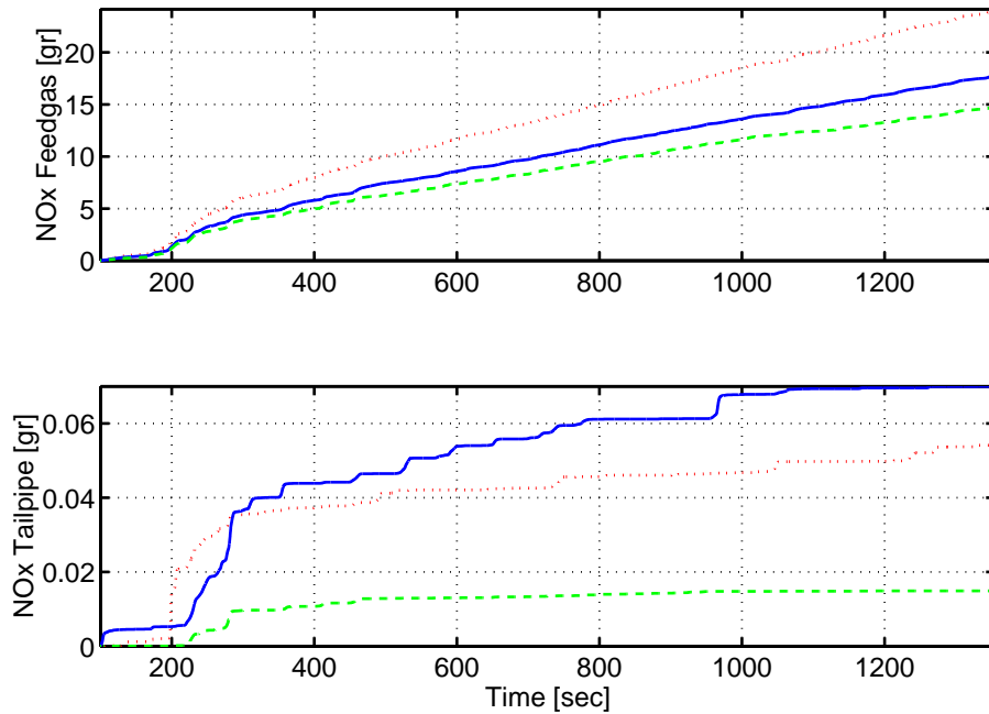
Fig. 28. 2.3L Engine. Pre- and Post-catalyst cumulative NOx emissions in grams at brick two. The dotted (red) refers to the controller with tailpipe A/F measured at Brick 1, solid line (blue) refers to the controller with tailpipe A/F measured at Brick 2 and the dot-dashed line (green) refers to the baseline controller.
