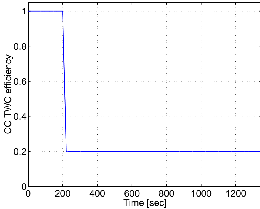
Fig. 17. Efficiency of the Close-Coupled TWC.
