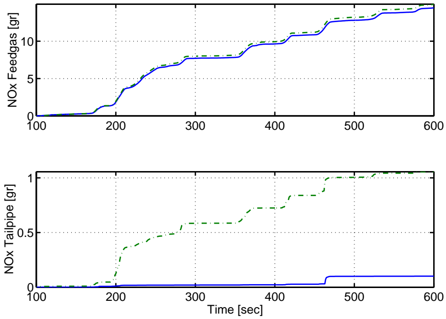
Fig. 25. 5.4L Engine. Pre- and Post-catalyst cumulative NO_x emissions in grams at brick one. The solid line (blue) refers to the dual UEGO controller and the dot-dashed line (green) to the baseline controller.
