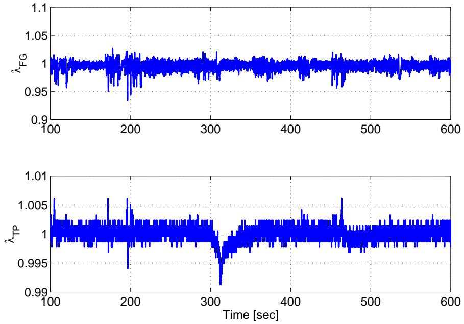
Fig. 21. 5.4L Engine. Air-Fuel ratio at feedgas and tailpipe.
