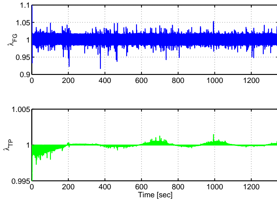
Fig. 9. Air-Fuel ratio at feedgas and tailpipe.
