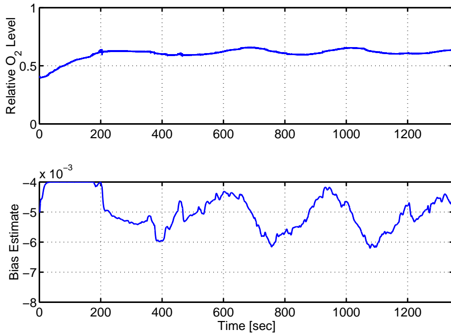
Fig. 11. Relative oxygen level and estimated bias.
