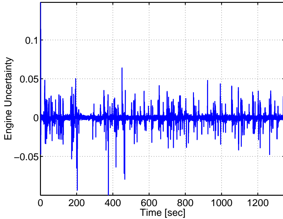
Fig. 3. Estimated uncertainty in the injected fuel quantity and in the estimated air-charge for a 5.4L engine over a drive cycle; units of normalized air-fuel ratio, \lambda .
