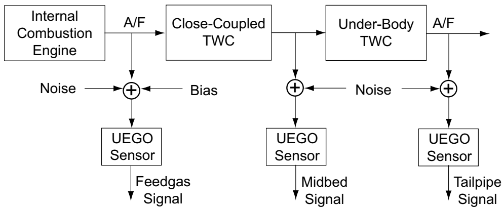
Fig. 12. Configuration with two catalysts.
