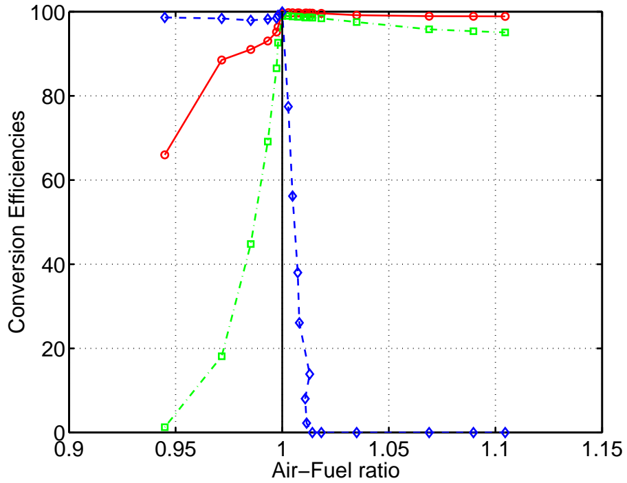
Fig. 5. Conversion efficiencies of HC (solid line) , CO (dot-dashed line), and NO_x (dashed line)
