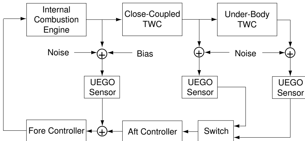
Fig. 16. Block diagram of the system formed by the cascade of the engine and the two catalytic converters regulated by the switching control in series configuration.
