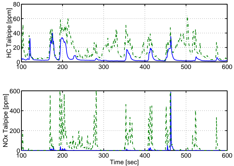
Fig. 22. 5.4L Engine. Post-catalyst HC and NO_x emissions in ppm at brick one. The solid line (blue) refers to the dual UEGO controller and the dot-dashed line (green) to the baseline controller.
