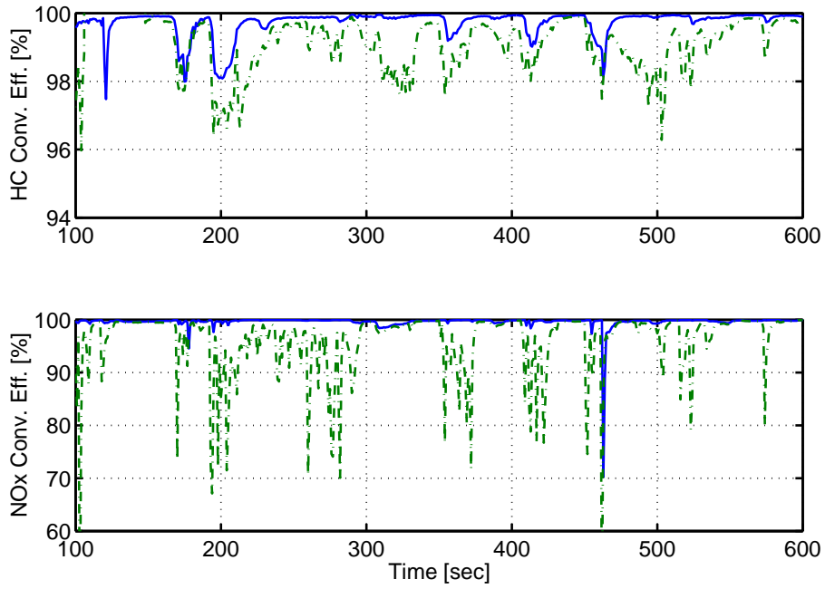
Fig. 23. 5.4L Engine. Instantaneous HC and NOx conversion efficiencies at brick one. The solid line (blue) refers to the dual UEGO controller and the dot-dashed line (green) to the baseline controller.
