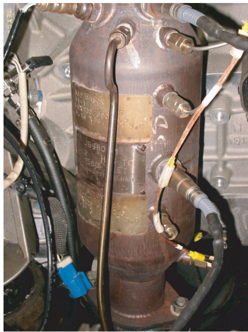
Fig. 19. Photograph of the TWC used on the 2.3L engine, viewed from the side. Feedgas is flowing from top to bottom. The feedgas emissions tap is visible at the top center of the photograph, feedgas UEGO and HEGO sensors are at the top left and right, and the brick one UEGO sensors is visible in the middle of the TWC.
