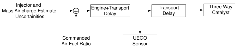
Fig. 2. Simplified engine model.
