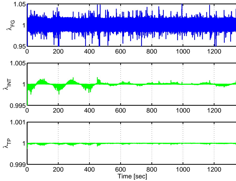
Fig. 13. Air-Fuel ratio respectively at feedgas, after the Close-Coupled TWC and tailpipe.
