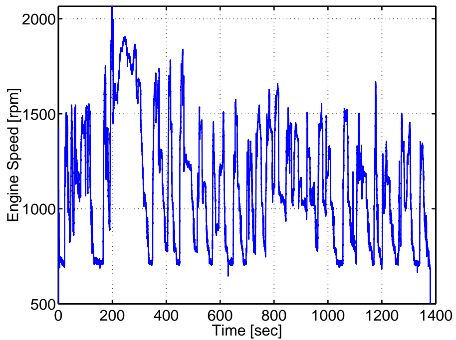
Fig. 20. Engine Speed over Test Cycle.
