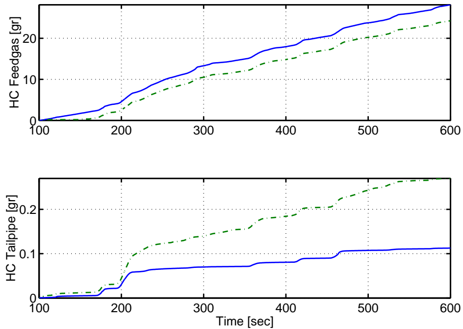
Fig. 24. 5.4L Engine. Pre- and Post-catalyst cumulative HC emissions in grams at brick one. The solid line (blue) refers to the dual UEGO controller and the dot-dashed line (green) to the baseline controller.
