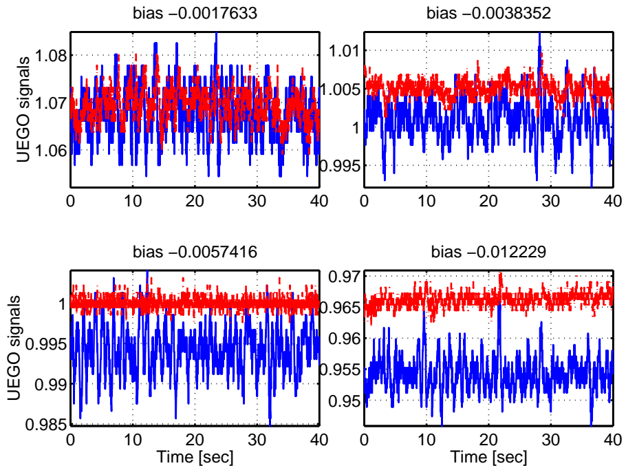
Fig. 6. Upstream (solid line) and downstream (dashed line) sensors output for different values of the air-fuel ratio. The engine speed and the load are constant.
