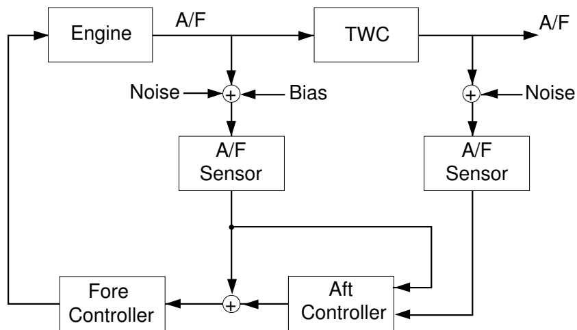
Fig. 8. Dual UEGO Fore-Aft Controller.
