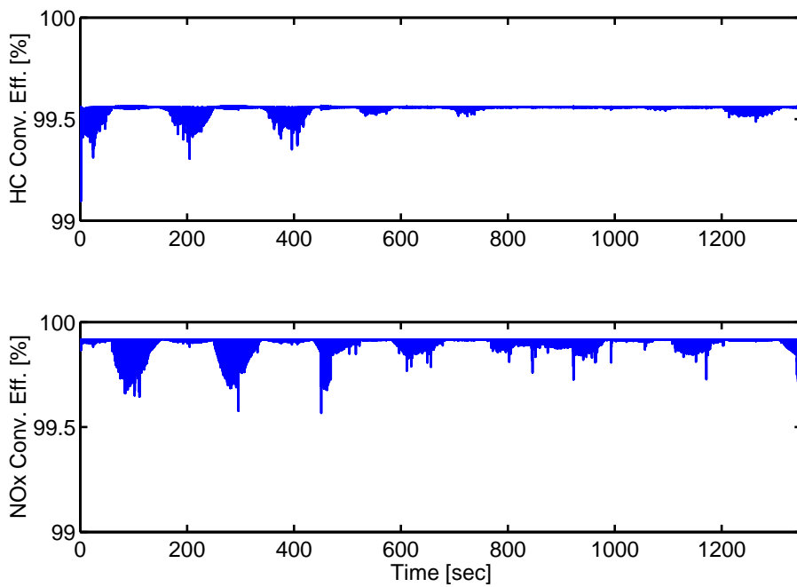
Fig. 14. Conversion efficiencies for unburned hydrocarbons and nitrogen oxide.
