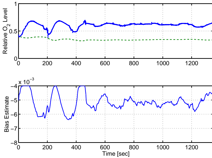
Fig. 15. Relative oxygen level of the CC-TWC (solid line) and the UB-TWC (dashed line), and estimated bias.
