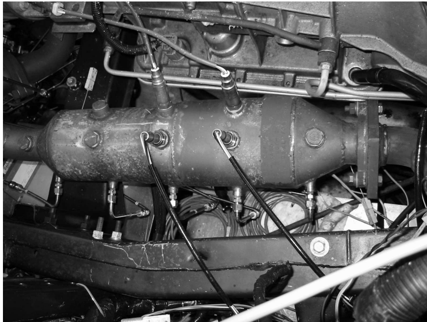
Fig. 18. Photograph of the TWC used on the 5.4L engine, viewed from the top. Feedgas is flowing from right to left. The emissions taps are visible at the bottom of the photograph, the UEGO sensors are in the middle, and the HEGO sensors are toward the top.
