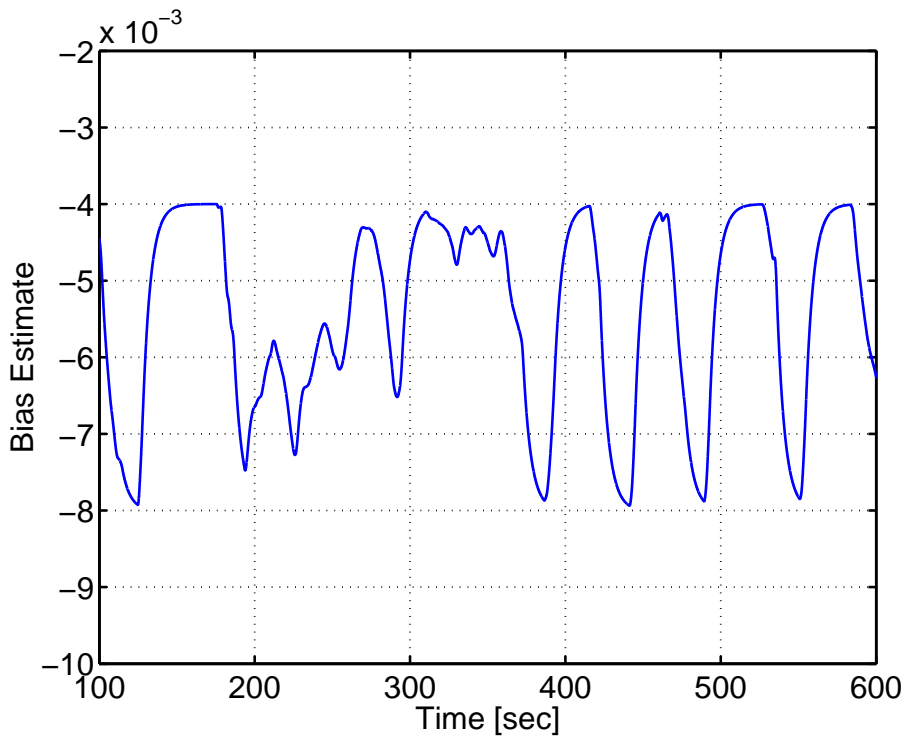
Fig. 26. 5.4L Engine. Bias estimate. Typical trace from 100 to 600 seconds when the UEGO is positioned at brick one.
