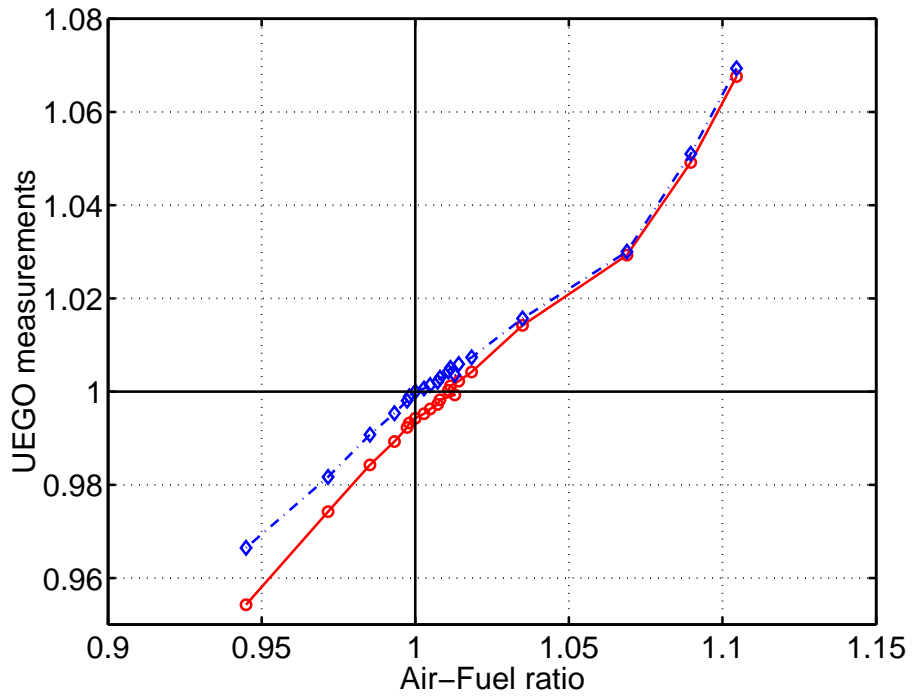
Fig. 7. Feedgas (solid line) and tailpipe (dashed line) UEGO sensors static curves.
