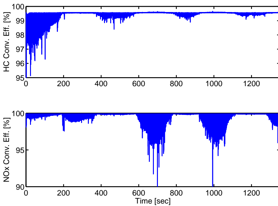
Fig. 10. Conversion efficiencies for unburned hydrocarbons and nitrogen oxide.
