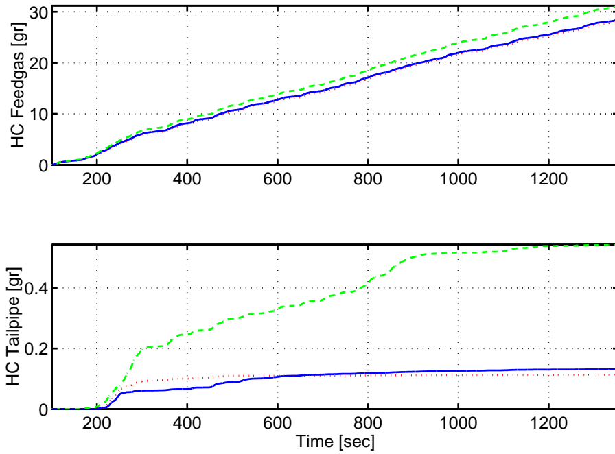
Fig. 27. 2.3L Engine. Pre- and Post-catalyst cumulative HC emissions in grams at brick two. The dotted (red) refers to the controller with tailpipe A/F measured at Brick 1, solid line (blue) refers to the controller with tailpipe A/F measured at Brick 2 and the dot-dashed line (green) refers to the baseline controller.
