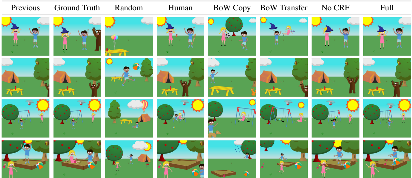
Figure 4. The proposed approach compared with the baselines on scenes selected from ones with consistent human ratings (top three rows success, final row failure). Simply copying the scene results in continuity errors (BOW Copy, Random), e.g., unrealistic disappearance of objects. Transferring the motions (BOW Transfer) or predicting without a CRF (No CRF) does not enforce consistency in scene dynamics (note the inaccurate motion of hat and sunglasses in the top row).
