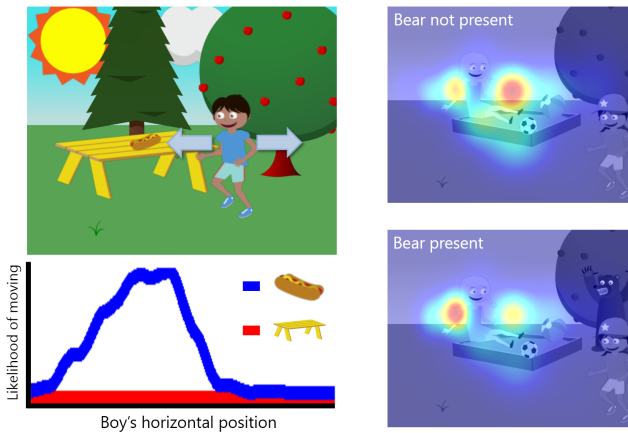
Figure 5. How do interactions influence predicted motion? (Left) We plot the relative likelihood \Omega that an object will move as we sweep the boy across the scene for the hot dog (blue) and picnic table (red). Notice the hot dog is more likely to move if the boy is near it. (Right) We show the distribution (red more likely; blue less likely) of the girl’s absolute motion \Upsilon_\omega in one scene (top) and if we just add a bear (bottom). Although there is a strong prior for moving forward, the bear’s presence overrides this.
