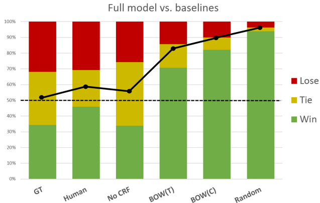
Figure 3. Human evaluation of the Full CRF predictions compared to the baselines (win, tie, lose.) The full method substantially outperforms the computer baselines and even crowdsourced human completions while doing comparably to the ground-truth scenes. The black line shows the win/loss ratio for each baseline.
