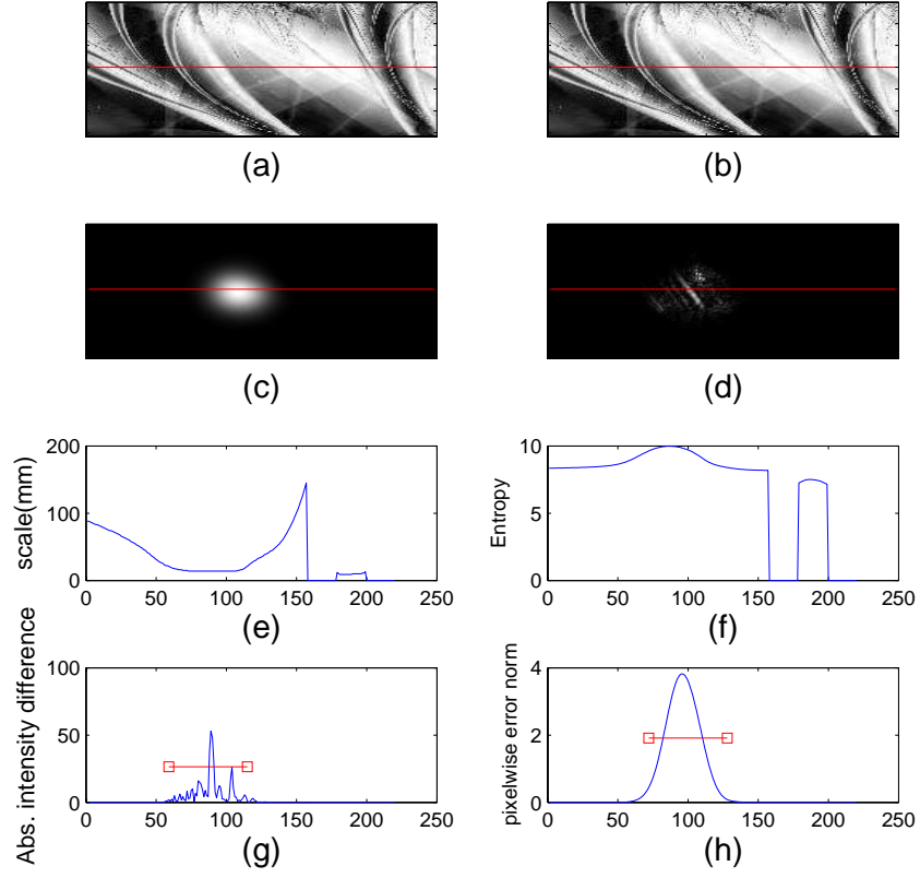
Figure 3. a) Target image, b) Floating image , c) Registration error norm, d) Absolute difference between images in a) and b), e) Significant spatial scale peaks, f) Joint entropy at scale peaks, g) Outer scale found(line)on intensity difference along line profile and h) Outer scale(line) on geometric error norm
