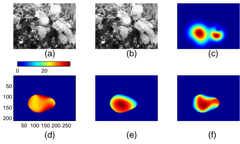
Figure 4. a) Target image, b) Floating image, c) geometric error norm, d) peaks in scale, e) joint entropy at peaks without gaussian scale space low pass filter and f) joint entropy at peaks with gaussian scale space filter
