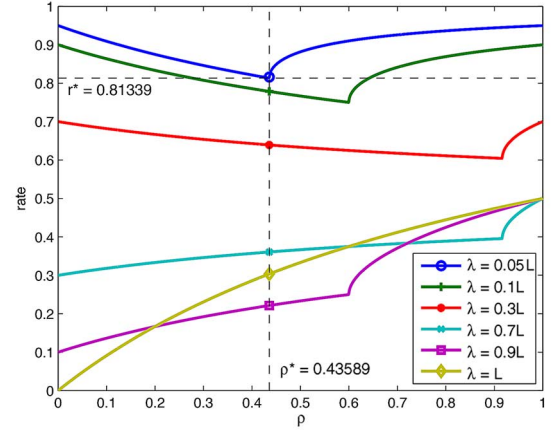
Fig. 1. Dominant roots r_i(\rho) of (41) and the optimal asymptotic convergence rate r^* \triangleq \min_{\rho} \{\max_i r_i(\rho)\} for a system with six distinct eigenvalues: 0.05L , 0.1L , 0.3L , 0.7L , 0.9L , and L .
