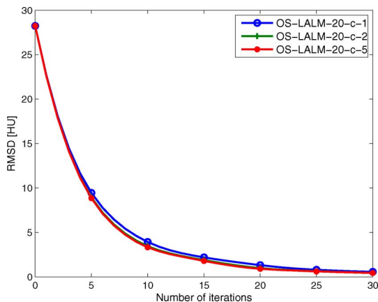
Fig. 5. Shoulder scan: rms differences between the reconstructed image \mathbf{x}^{(k)} and the reference reconstruction \mathbf{x}^* as a function of iteration using the proposed algorithm with different number of FISTA iterations n (1, 2, and 5) for solving the inner constrained denoising problem.
