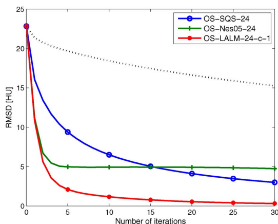
Fig. 8. GE performance phantom: rms differences between the reconstructed image \mathbf{x}^{(k)} and the reference reconstruction \mathbf{x}^* as a function of iteration using OS-based algorithms with 24 subsets. Dotted line shows the rms differences using the standard OS algorithm with one subset.
