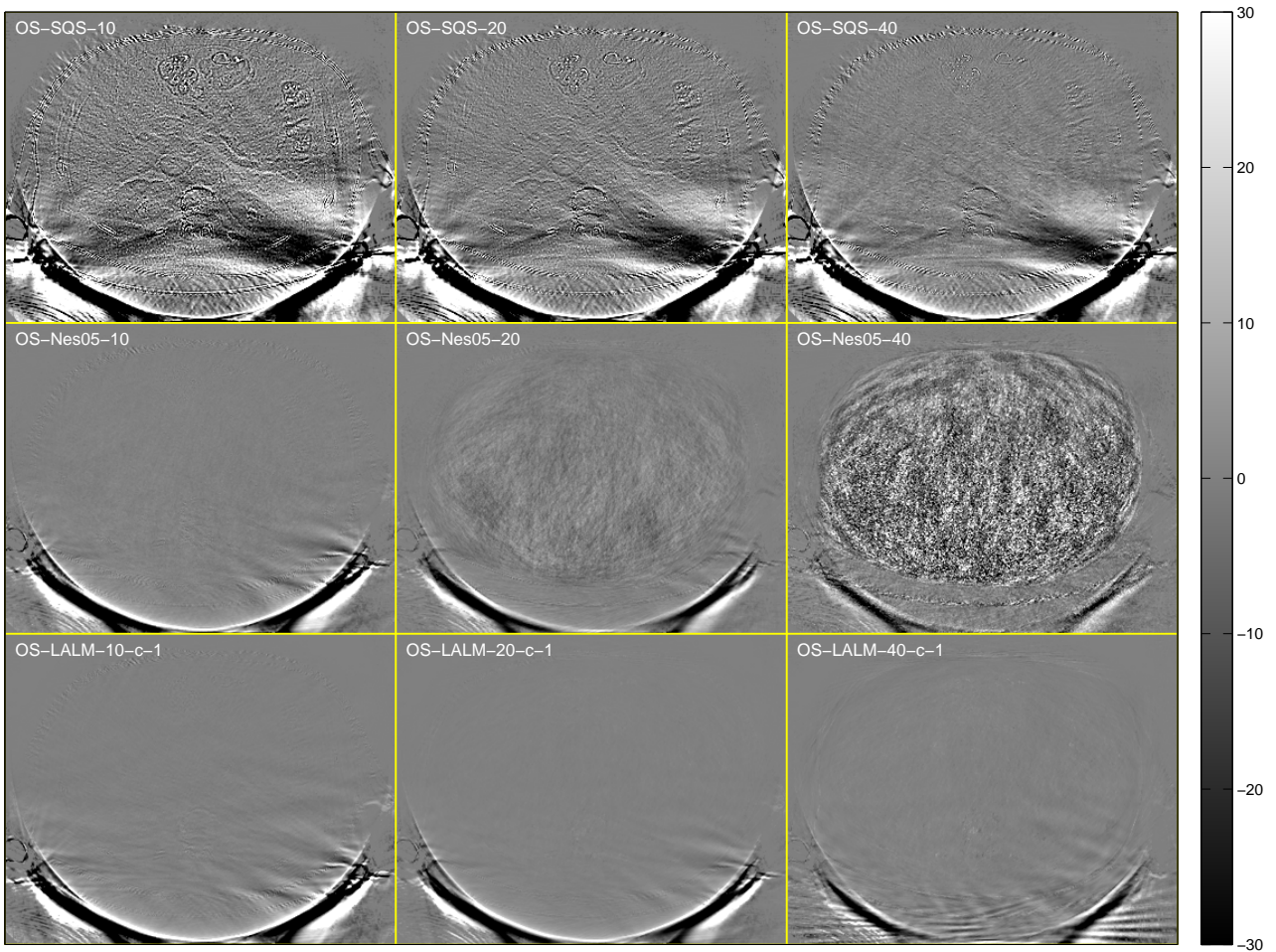
Fig. 7: Truncated abdomen scan: cropped difference images (displayed from -30 to 30 HU) from the central transaxial plane of \mathbf{x}^{(30)} - \mathbf{x}^* using OS-based algorithms.
