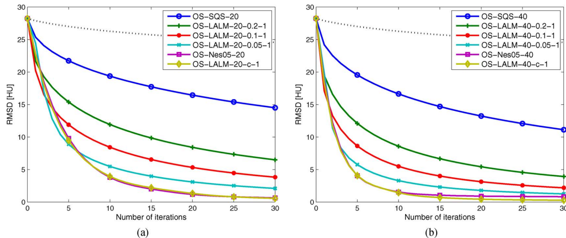
Fig. 4. Shoulder scan: rms differences between the reconstructed image \mathbf{x}^{(k)} and the reference reconstruction \mathbf{x}^* as a function of iteration using OS-based algorithms with (a) 20 subsets and (b) 40 subsets, respectively. Dotted lines show the rms differences using the standard OS algorithm with one subset.
