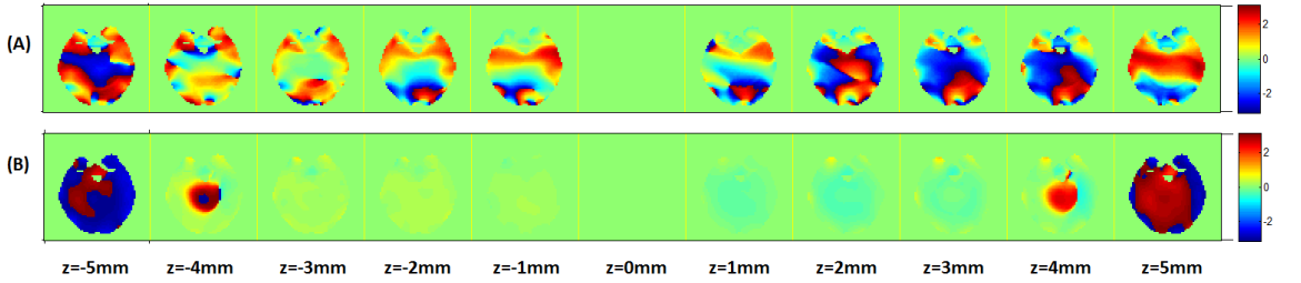
Figure 6.4: Transverse magnetization phase along z axis by different RF pulses. Top row (A) shows the transverse magnetization from the scaled version of a small tip-angle pulse, and the bottom row (B) shows our proposed large tip-angle RF pulse design. The large tip-angle design method shows much smaller phase variation, implying less signal loss in the reconstructed image.
