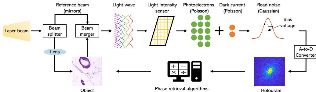
Figure 1: Illustration of Poisson and Gaussian noise statistics in holographic phase retrieval.
