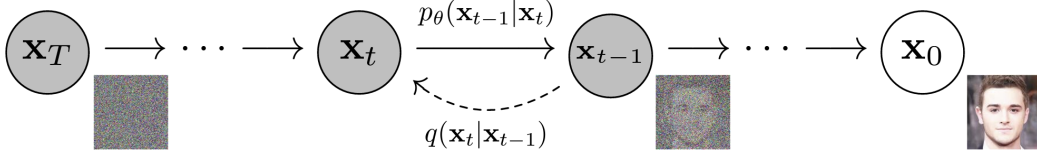
Figure A.2: The DDPM framework, adopted from [58].
