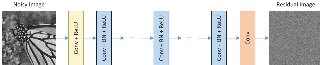
Figure A.1: The architecture of the adopted DnCNN network [96].
