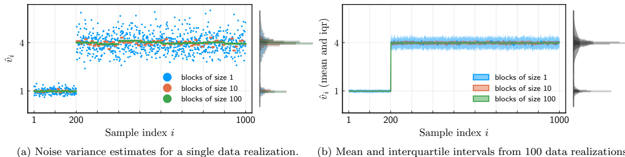
Figure 7: Estimated noise variances for varying block sizes.
