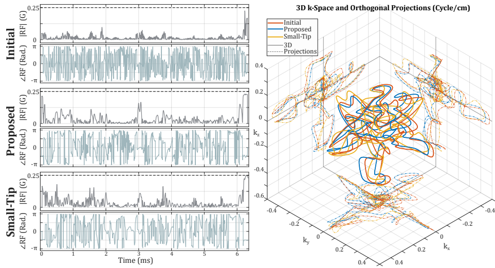
Fig. S1. OV saturation pulses for the cuboid IV, designed with our approach (Proposed) and Sun’s small-tip method (experiment OV90 in the main manuscript). The left panel shows the RF waveforms. The right panel shows the 3D k-space trajectories and their orthogonal projections: The three trajectories explore largely overlapping regions in excitation k-space.
