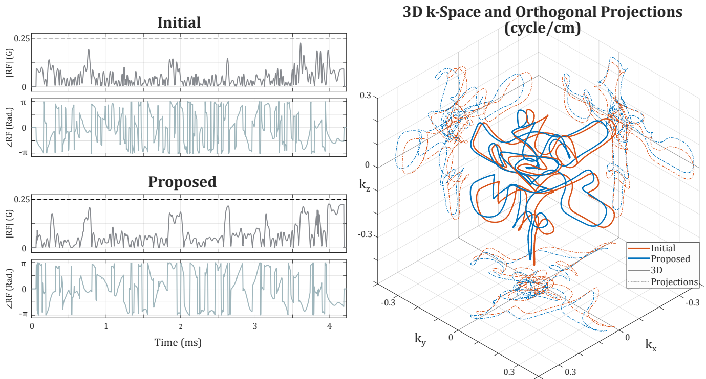
Fig. S3. Cuboid IV inversion (experiment IV180 in the main manuscript). The left panel compares the RF waveforms of the initial and optimized (Proposed) pulses. The right panel compares the k-space trajectories of the two pulses.
