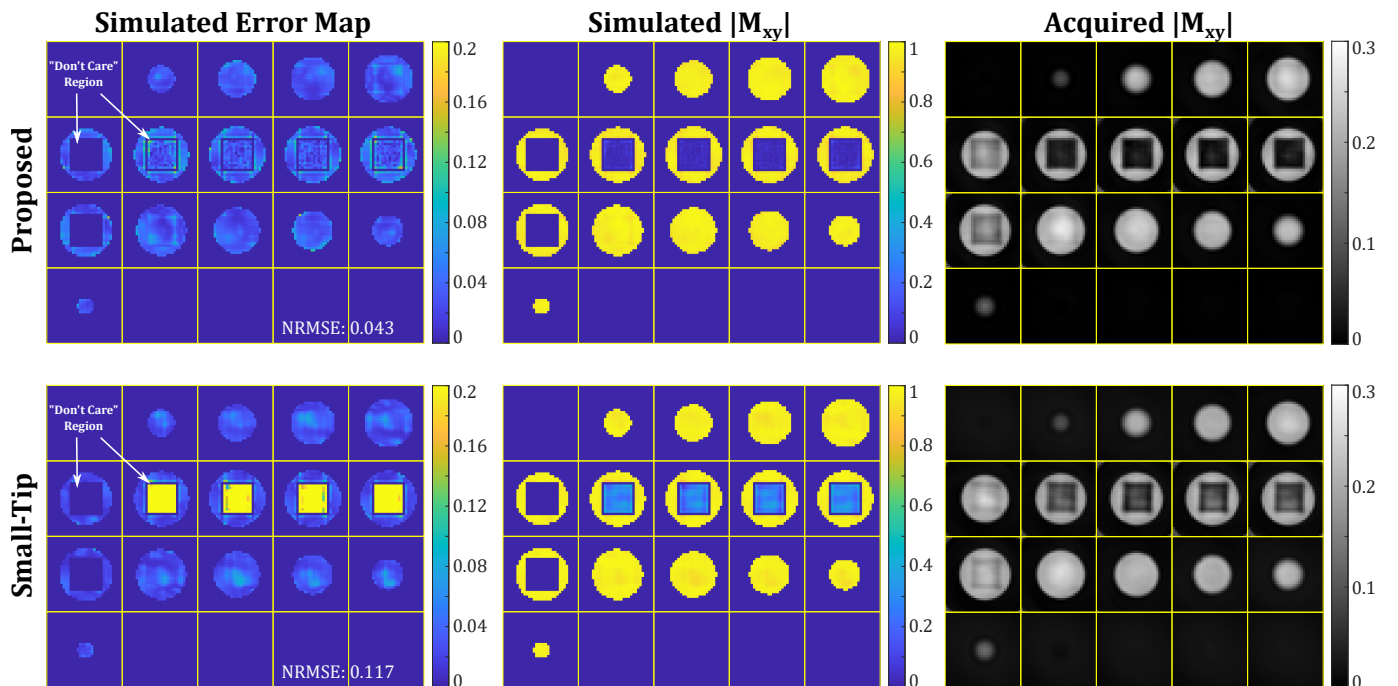
Fig. 5. Experimental validation of the pulses shown in Fig. 4. The left panel shows the error map from simulation. Our approach has much smaller ( \sim 63\% ) NRMSE in simulation compared to Small-Tip. Acquired results (right) agree with the simulations (middle). Small-Tip approach has larger error inside the IV: This is expected, as the method produces only small-tip pulses, that we then scaled to meet the large-tip objective. The scaling increases excitation error inside IV while reducing error in the OV. Our approach directly designs large-tip pulses without this type of ‘scaling’ error.
