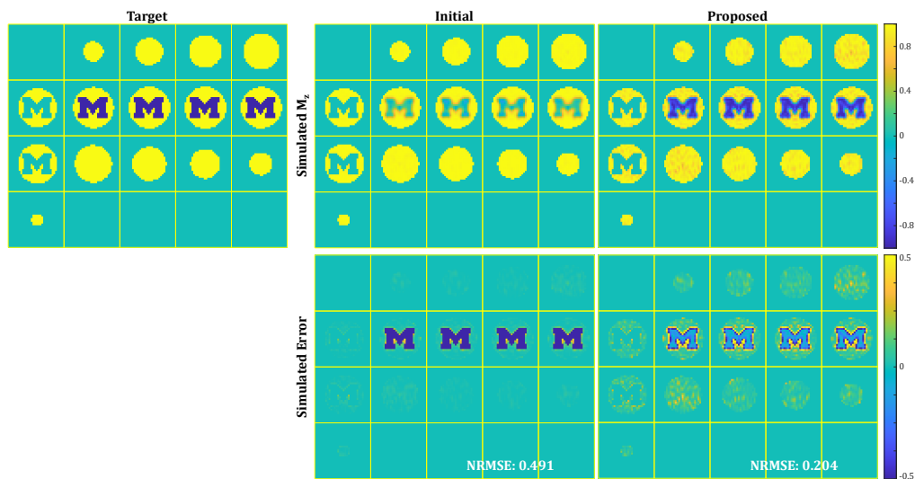
Fig. S6. Simulated excitation patterns for the pulses shown in Fig. S5.
