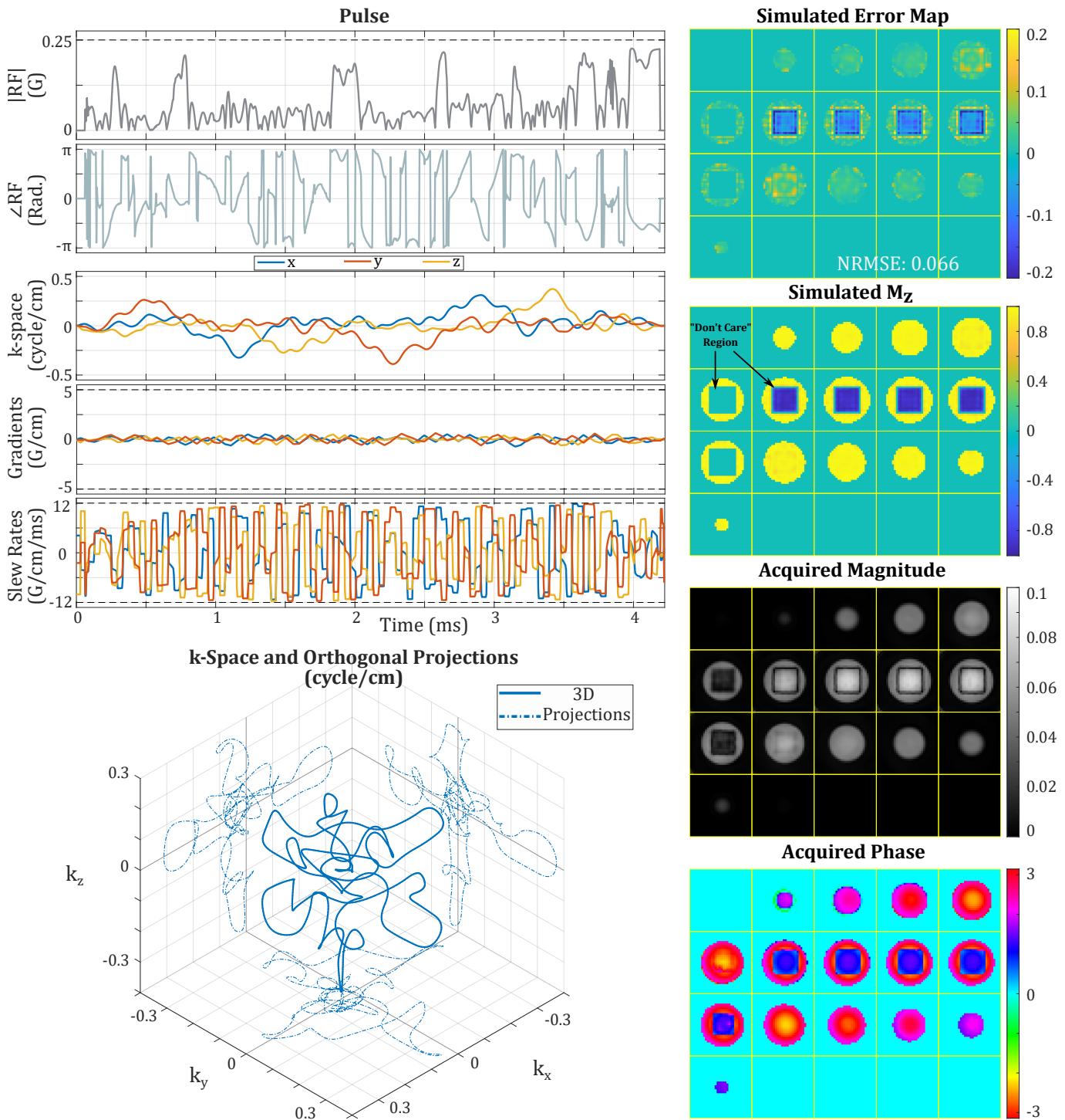
Fig. 6. IV inversion results for the cuboid IV pattern (Experiment IV180). As desired, the 4.2 ms pulse satisfies all constraints. The gradient waveform is again far from its peak constraint of 5 G/cm. Compared to the OV90 experiment, the pulse has more extreme slew rate waveforms. The acquired magnitude and phase (i.e., the “observed inversion”) were obtained with the sequence in Fig. 2. We observe good agreement between simulated and acquired inversion patterns. The designed pulse successfully inverts the IV, as indicated by similar magnitude image intensity in the IV and OV regions (apart from transmit/receive coil shading) and a \pi phase shift across the IV/OV boundary. The dark bands in the acquired images at the IV/OV boundary are due to spin saturation from incomplete inversion (and overlap substantially with the prescribed “don’t care” region).
