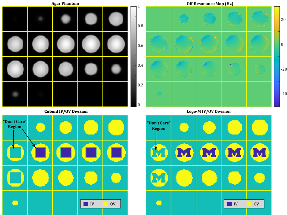
Fig. 3. Experimental phantom, and the two target patterns (IV/OV divisions) used in our experiments. Top left: Magnitude image of the uniform Agar phantom. Top right: Observed field map, used in the pulse design to account for B0 inhomogeneity. A conservative mask that is 1-voxel-wide larger than the phantom support was used to ensure that the phantom boundary was included in the design. This expanded mask is the likely cause for the relatively large B0 values in some pixels at the edge of the mask (that are likely just outside the phantom). Bottom: Cuboid (left) and “block-M” (right) target patterns. We prescribed a “don’t care” (region with arrows) at the boundary between the IV and OV regions that is excluded when calculating the design loss. For the cuboid pattern, the don’t care region included the entire 3D IV/OV boundary, whereas for the block-M pattern, only the top and bottom slices (slices 6 and 11; slice numbers increase left-to-right and top-to-bottom) were included due to the low in-plane spatial resolution of the design grid.
