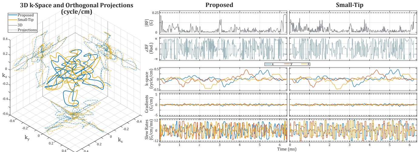
Fig. 4. OV saturation pulses for the cuboid IV (Fig. 3), designed with our approach (Proposed) and the small-tip method in [12] (experiment OV90). The left panel shows the 3D k-space trajectories and their orthogonal projections: The two trajectories explore largely overlapping regions in excitation k-space. The right two panels show RF, gradient, and slew rate waveforms. Both designs satisfy the constraints, but for the small-tip design it was necessary to apply the VERSE [25] algorithm near the end of the pulse (see Discussion). Gradient peak amplitudes remain quite small, whereas the gradient slew rates are frequently near their limit.
