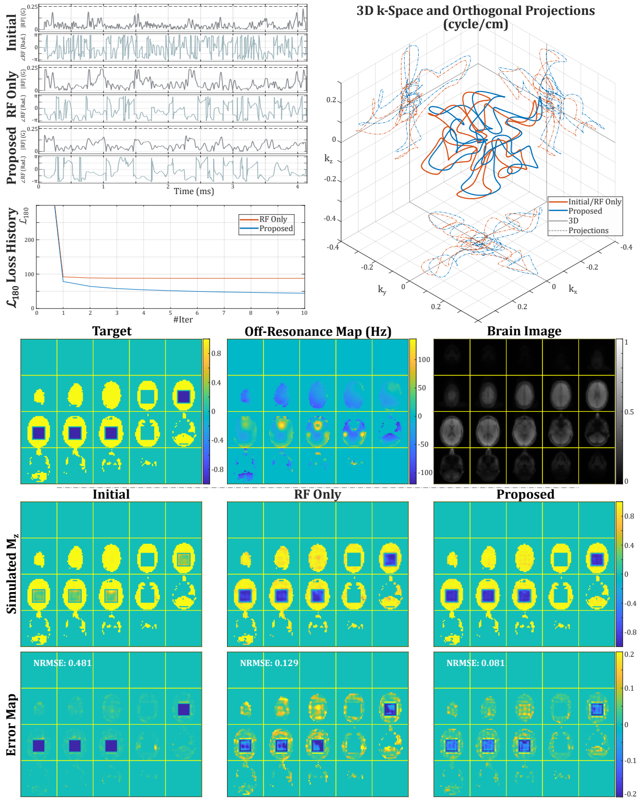
Fig. S7. Cuboid IV inversion based on a B_0 (off-resonance) map obtained in a volunteer. Three pulses are compared: (1) Initial, (2) 'RF Only', obtained by keeping the gradients fixed at their initial shapes and optimizing only the RF waveform with the proposed auto-differentiation approach, and (3) the proposed jointly optimized pulse. While our optimized k-space trajectory is similar to the initial k-space trajectory, the jointly optimized pulse (Proposed) attains an excitation accuracy (NRMSE: 8.1%) that is 37% better than the 'RF Only' pulse (NRMSE: 12.9%). This improvement is also reflected in the convergence ( \mathcal{L}_{180} loss history) plot.
