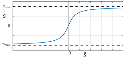
Fig. 1. Turning constrained slew rate s into unconstrained \tilde{s} , by change of variable \tan^{-1} .
