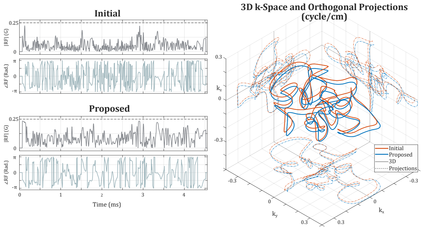
Fig. S5. Block-M IV inversion pulse (experiment IV180M in the main manuscript). The left panel compares the RF waveforms of the initial and optimized (Proposed) pulses. The right panel compares the k-space trajectories of the two pulses.
