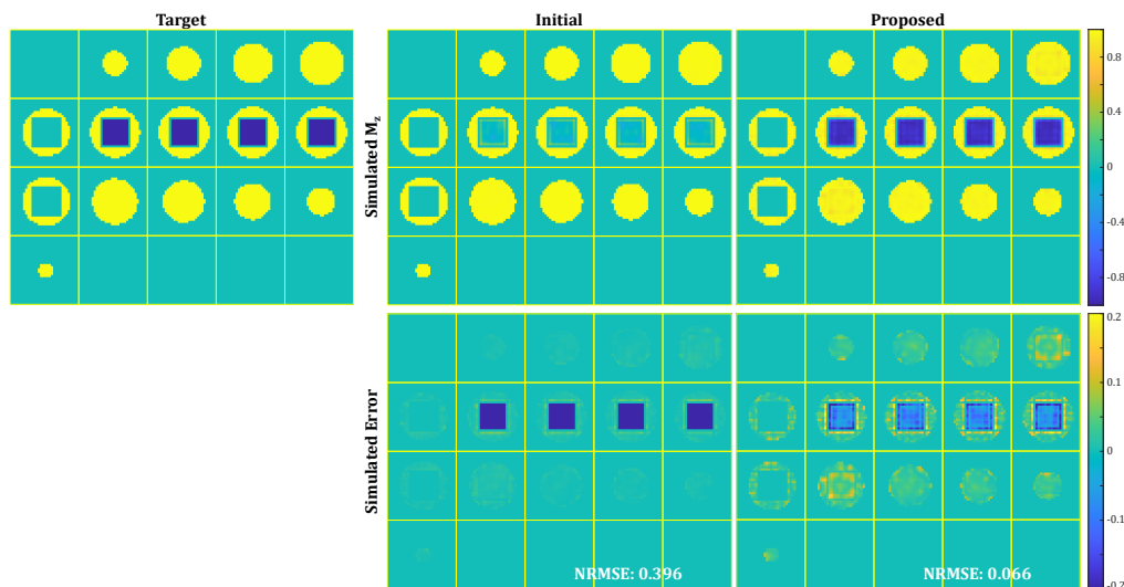
Fig. S4. Simulated excitation patterns for the pulses shown in Fig. S3.
