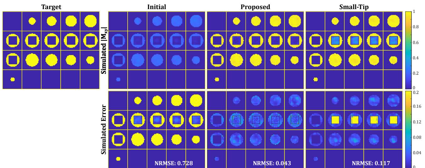
Fig. S2. Simulated excitation patterns for the pulses shown in Fig. S1. Both our method and the Small-Tip method have significantly improved excitation accuracy when compared to the initial pulse. Our approach has much smaller (-63%) NRMSE in simulation compared to Small-Tip. Small-Tip approach has larger error inside the IV: This is expected, as the method produces only small-tip pulses, that we then scaled to meet the large-tip objective. The scaling increases excitation error inside IV while reducing error in the OV. Our approach directly designs large-tip pulses without this type of ‘scaling’ error.
