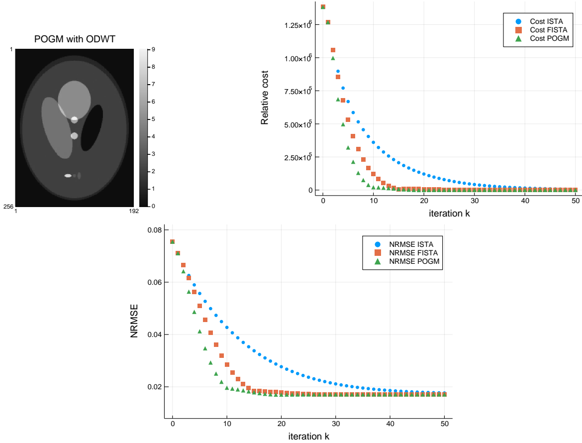
Fig. 2. Comparison of ISTA/PGM, FISTA/FPGM and POGM for single-coil MRI reconstruction with orthogonal discrete wavelet transform sparsity regularizer using the 1-norm. Minimizer \hat{\mathbf{x}} of (7); cost function for (7); NRMSE versus iteration k . FISTA requires about 40% more iterations to converge than POGM, consistent with the 2\times better worst-case bound of POGM.
