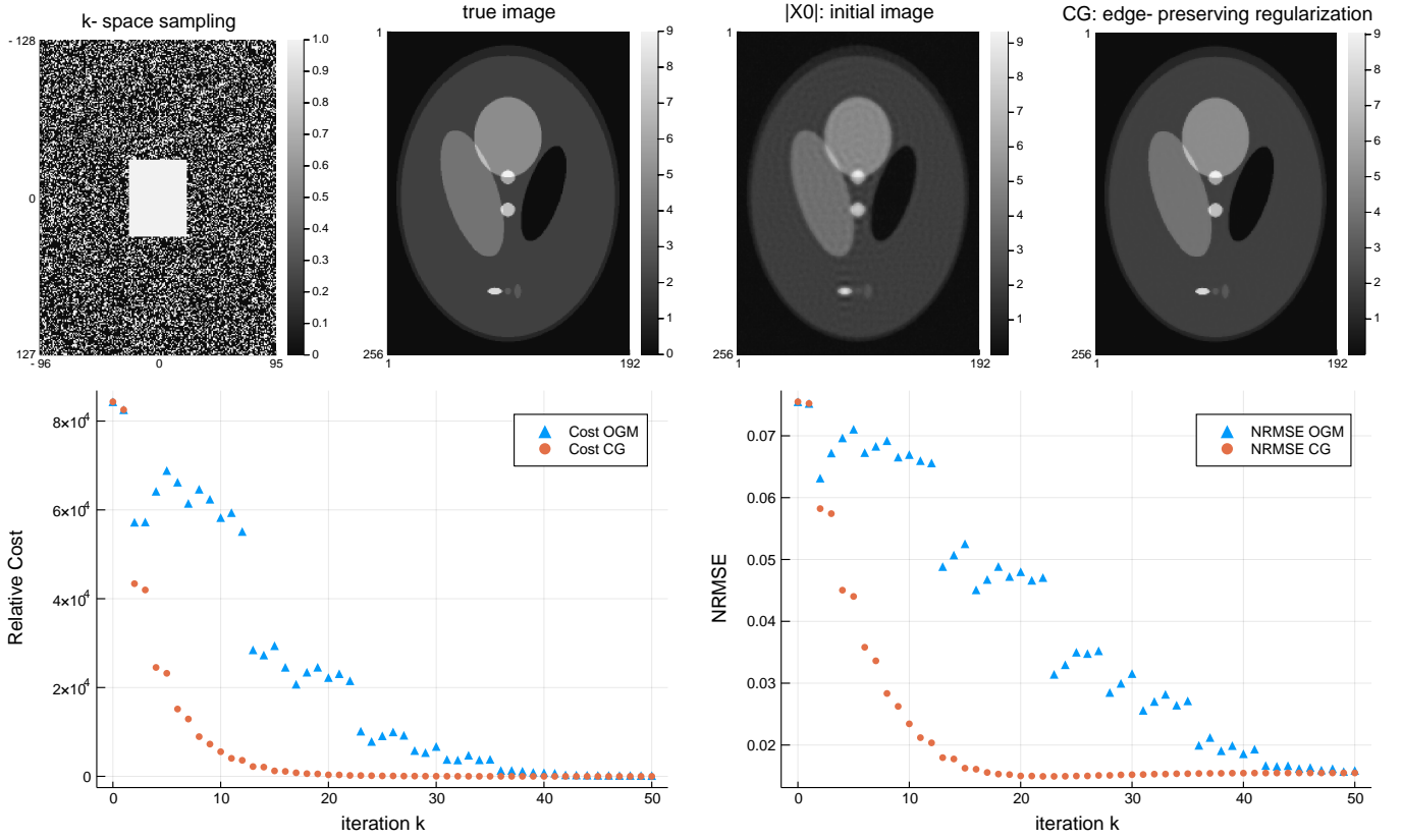
Fig. 1. Comparison of CG and OGM convergence for single-coil MRI reconstruction with edge-preserving regularization (akin to anisotropic TV with corner rounding). From left to right: Top row: k-space sampling pattern where only 34% of the phase-encodes are collected, true image, initial image from zero-filled k-space data, minimizer \hat{x} of (6). (Both CG and OGM converge to the same limit \hat{x} .) Bottom row: cost function \Psi(x_k) in (6) and normalized root mean squared error (NRMSE) \|x_k - x\|_2 / \|x\|_2 versus iteration k .
