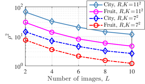
Fig. 1. Empirical values of \rho^2 in (7) show a decrease with L for different datasets and filter dimensions. (The fruit and city datasets with L = 10 and N = 10^4 [1] were preprocessed with contrast enhancement and zero-mean subtraction [1], [2]. For L < 10 , the results are averaged over 50 datasets randomly selected from the full datasets.) Under the assumptions of Corollary 3.2, the decrease in this quantity leads to a better expected error bound in (5). Without preprocessing, the quantity \rho^2 increases by a factor of around 10^3 .
