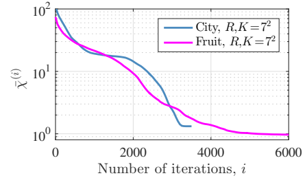
Fig. 2. Empirical estimate of \bar{\chi} in (11) across iterations in the alternating optimization algorithm [1] that solves CAOL (P0) with \alpha = 10^{-3} . (The fruit and city datasets with L = 10 and N = 10^4 [1] were preprocessed with contrast enhancement and zero-mean subtraction [1], [2]. The model mismatches \{E_l^{(i)} : \forall l\} at the i th iteration were calculated every 50 iterations based on (3), where we use the converged filters for D_{\text{true}} .) When \bar{\chi} is small, the high probability error bound (9) in Theorem 3.3 depends primarily on \bar{\rho} defined in (11).
