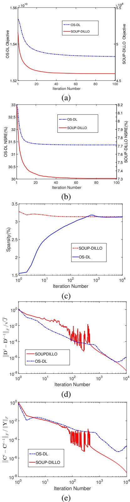
Fig. 7. Convergence behavior of the SOUP-DILLO and OS-DL Algorithms for (P1) and (P2): (a) Objective function; (b) Normalized sparse representation error (percentage); (c) sparsity factor of \mathbf{C} ( \sum_{j=1}^J (\|\mathbf{c}_j\|_0 / nN) – expressed as a percentage); (d) normalized changes between successive \mathbf{D} iterates ( \|\mathbf{D}^t - \mathbf{D}^{t-1}\|_F / \sqrt{J} ); and (e) normalized changes between successive \mathbf{C} iterates ( \|\mathbf{C}^t - \mathbf{C}^{t-1}\|_F / \|\mathbf{Y}\|_F ). Note that (a) and (b) have two vertical scales.
