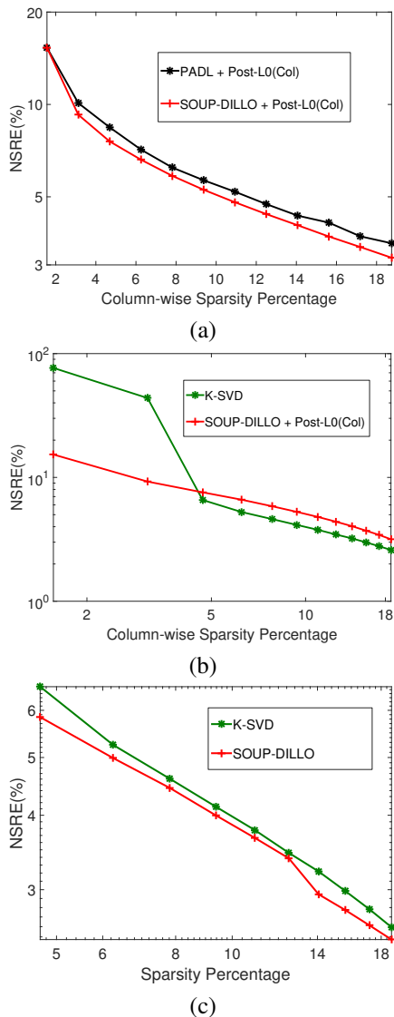
Fig. 8. Comparison of dictionary learning methods for adaptive sparse representation (NSRE [84] expressed as percentage): (a) NSRE values achieved with column-wise sparse coding (using orthogonal matching pursuit) using dictionaries learned with PADL [90], [91] and SOUP-DILLO; (b) NSRE values obtained using K-SVD [93] compared to those with column-wise sparse coding (as in (a)) using learned SOUP-DILLO dictionaries; and (c) NSRE values obtained by SOUP-DILLO in Problem (P1) compared to those of K-SVD at matching net sparsity factors. The term ‘Post-L0(Col)’ in the plot legends denotes (post) column-wise sparse coding using learned dictionaries.
