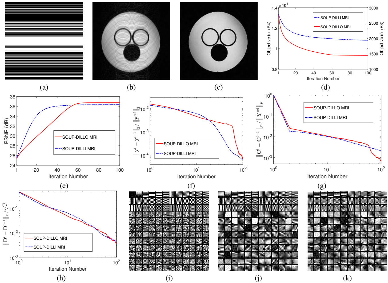
Fig. 5. Behavior of SOUP-DILLO MRI (for (P3)) and SOUP-DILLI MRI (for (P4)) for Image (c) with Cartesian sampling and 2.5x undersampling: (a) sampling mask in k-space; (b) magnitude of initial reconstruction \mathbf{y}^0 (PSNR = 24.9 dB); (c) SOUP DILLO MRI (final) reconstruction magnitude (PSNR = 36.8 dB); (d) objective function values for SOUP-DILLO MRI and SOUP-DILLI MRI; (e) reconstruction PSNR over iterations; (f) changes between successive image iterates ( \|\mathbf{y}^t - \mathbf{y}^{t-1}\|_2 / \|\mathbf{y}^{\text{ref}}\|_2 ) normalized by the norm of the reference image ( \|\mathbf{y}^{\text{ref}}\|_2 = 122.2 ); (g) normalized changes between successive coefficient iterates ( \|\mathbf{C}^t - \mathbf{C}^{t-1}\|_F / \|\mathbf{Y}^{\text{ref}}\|_F ) where \mathbf{Y}^{\text{ref}} is the patch matrix for the reference image; (h) normalized changes between successive dictionary iterates ( \|\mathbf{D}^t - \mathbf{D}^{t-1}\|_F / \sqrt{J} ); (i) initial real-valued dictionary in the algorithms; and (j) real and (k) imaginary parts of the learnt dictionary for SOUP-DILLO MRI. The dictionary columns or atoms are shown as 6 \times 6 patches.
