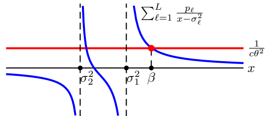
Fig. 4: Location of the largest root \beta of B(x) for \lambda = 0.7 (i.e., \sigma_1^2 = 2.04 and \sigma_2^2 = 0.874 ), c = 10 , p = (0.7, 0.3) and \theta = 1 .
