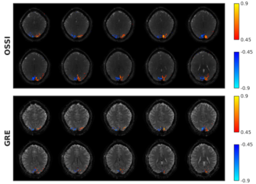
Figure 4. 3D OSSI and GRE activation maps of the central 10 slices. The backgrounds of the activation maps are means of the reconstructed images, activation threshold of 0.45, and a continuity threshold of 2 is applied. 3D OSSI presents 2.2 times more activated voxels at the lower third of the brain compared to multi-slice GRE imaging at TE = 30 ms.
