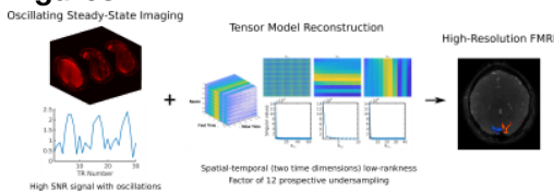
Figure 1. OSSI images with oscillations and high SNR can be structured to have two time dimensions. Together with a tensor model that exploits the spatial-temporal low-rankness for all the matrix unfoldings, the proposed work enables a factor of 12 acquisition acceleration and provides high-resolution fMRI results.
