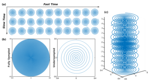
Figure 2. (a) Prospective 2D undersampling with pseudo-randomized Golden-angle rotations between the oscillation dimension ("fast time") and the fMRI time dimension ("slow time"). (b) The undersampled variable-density spiral trajectory for each frame or each k z plane with a factor of 12 acceleration compared to fully sampled. (c) 3D stack-of-spirals undersampling pattern with one spiral for the outer k-space planes and two spirals for the two central k z planes representing a factor of 10 acceleration.
