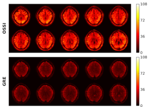
Figure 5. 3D OSSI and GRE temporal SNR maps of the central 10 slices. Compared to multi-slice Ernst angle GRE imaging, 3D OSSI presents 2.2 times larger average temporal SNR within the brain.
