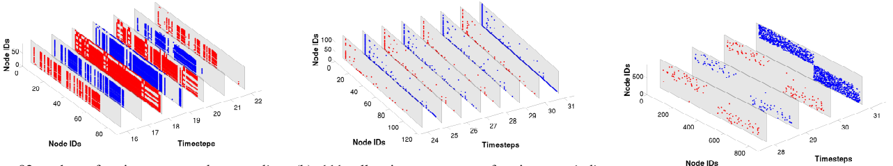
(g) 82 authors forming a ranged near clique on DBLP, with burgeoning collaboration from star appearing strongly on odd numbered days, especially Dec. 25 and 31 (h) 111 callers in Phonenumber forming a periodic near bipartite core appearing strongly on Dec. 31 (i) 792 callers in Phonenumber forming a oneshot near bipartite core appearing strongly on Dec. 31
