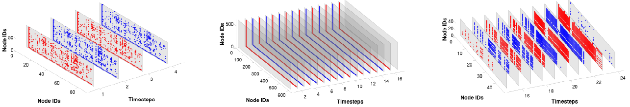
(d) 82 users in Yahoo-IM forming a constant star over the observed 4 weeks (e) 589 honeypot machines were attacked on Honeynet over 2 weeks, forming a ranged star (f) 43 authors that publish together in biotechnology journals forming a ranged near clique on DBLP
