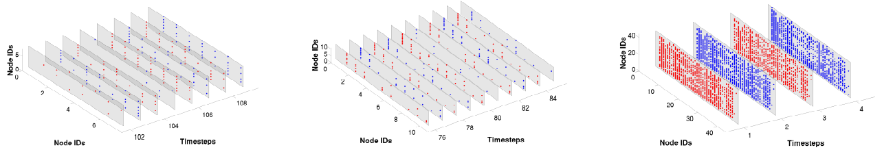
(a) 8 employees of the Enron legal team forming a flickering near clique (b) 10 employees of the Enron legal team forming a flickering star with the boss as the hub (c) 40 users in Yahoo-IM forming a constant near clique with 55% density over the observed 4 weeks
