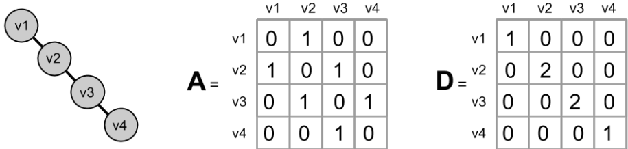
Figure 2.7: A chain of 4 nodes, and its adjacency and degree matrices.
