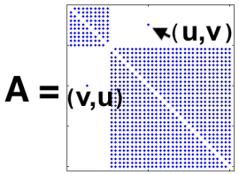
Figure 2.6: Adjacency matrix of a simple, unweighted and undirected graph.
