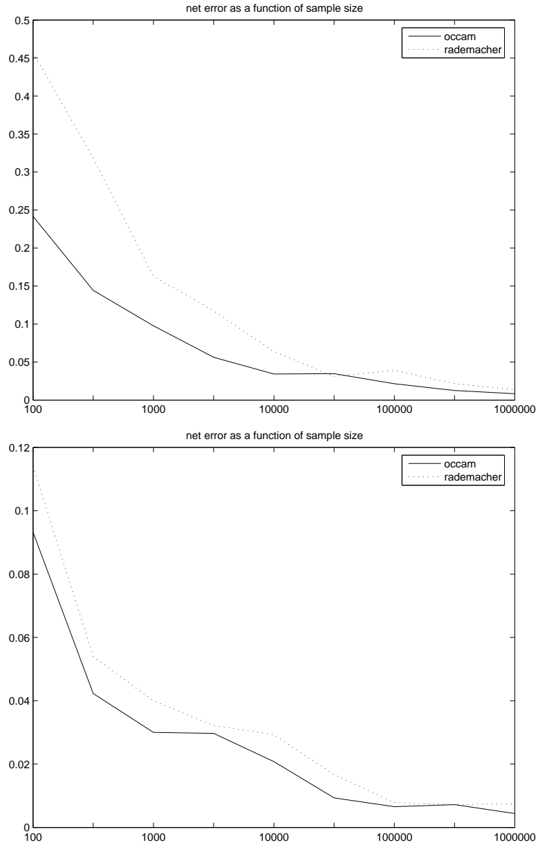
Figure 6: The error \mathcal{M}(\widehat{G}_{\mathcal{G},\alpha}) as a function of sample size for the histogram experiments in Section 7.1. All results are averaged over 100 repetitions for each training sample size. (Top) Results for the original MV-SRM algorithm ( \nu = 1 ). (Bottom) Results for \nu = 0 . In this case the error is more evenly distributed between mass and volume, whereas in the former case all the error is in the mass term.
