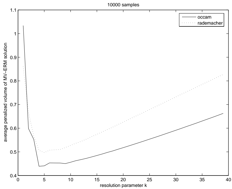
Figure 7: The penalized volume of the MV-ERM estimates G_{\mathcal{G},\alpha}^k , as a function of k , where 1/k is the sidelength of the histogram cell. The results are for a sample size of 10000. Results represent an average over 100 repetitions. Clearly, the Occam's razor bound is smaller than the Rademacher penalty (look at the right side of the plot), to which we may attribute its improved performance (see Figure 6).
