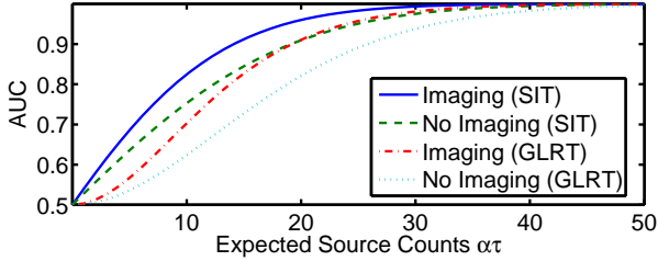
Fig. 4: AUC versus expected source counts for a circular uniform-sensitivity detector with \lambda_b\tau = 100 and \mu r = 5 .
