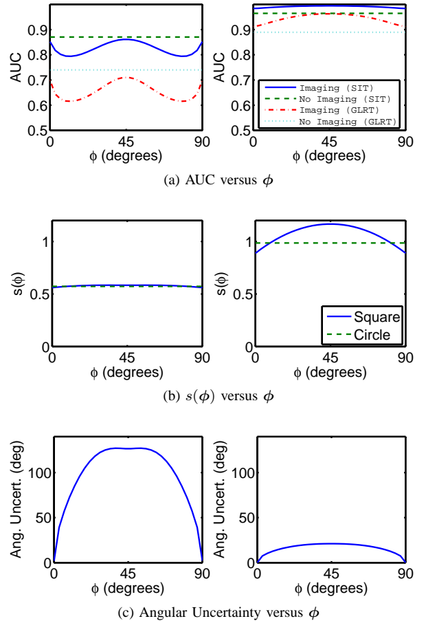
Fig. 5: AUC, relative sensitivity, and angular uncertainty for square position-sensitive and circular counting detectors of equal area ( r = 2l/\sqrt{\pi} ) vs. \phi with \mu l = 0.5 (left) and \mu l = 5 (right), and \alpha\tau = \lambda_b\tau = 10 .
