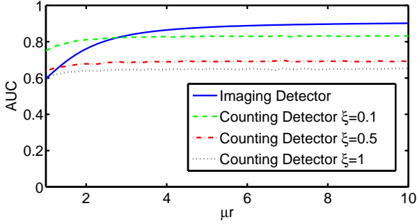
Fig. 8: AUC vs. \mu r for position-sensitive and counting detectors, where the counting detector uses a “guessed” background rate in the “known background” GLRT. \alpha\tau = \lambda_b\tau = 10 .
