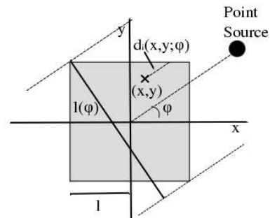
Fig. 2: Diagram of square detector with side length 2l .
