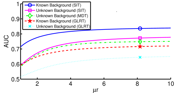
Fig. 7: AUC for spatially uniform background of known and unknown intensity versus attenuation–radius product for \alpha \tau = 10 , \lambda_b \tau = 100 .
