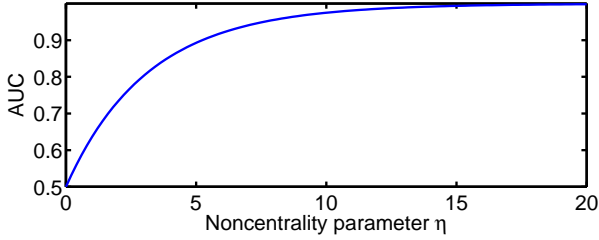
Fig. 1: AUC of GLRT (14) versus noncentrality parameter \eta of the asymptotic distribution of the GLRT.
