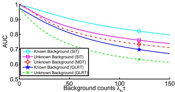
Fig. 6: AUC vs. \lambda_b \tau for spatially uniform background of known and unknown intensity background where \mu r = 10 and \alpha \tau = 10 .
