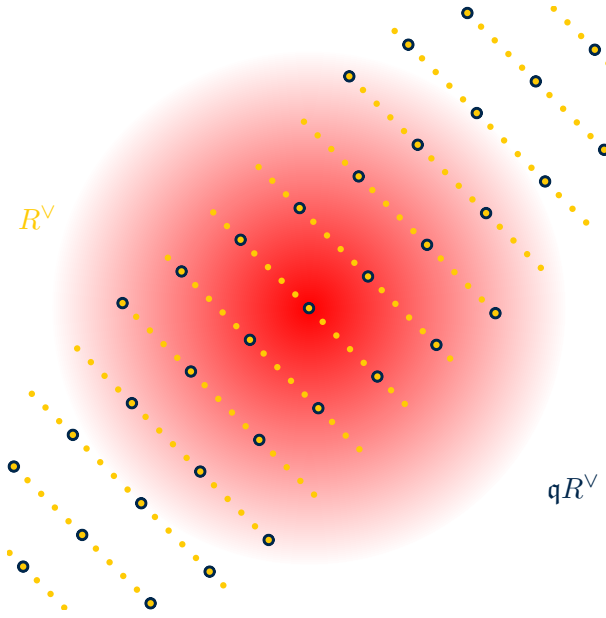
Figure 7: The canonical embedding of: (in maize) the dual ideal R^\vee = (2\zeta)^{-1}R of the ring R = \mathbb{Z}[\zeta] for \zeta = \sqrt{11} , (in blue) the ideal qR^\vee where q = (1 + \zeta)R + 5R is a prime ideal of norm N(q) = 5 , and (in red) a spherical Gaussian of parameter r = 2 . Notice that the Gaussian is “well spread” relative to R^\vee and even qR^\vee , as implied by Theorem 5.2. The “tweak” factor 2\zeta that maps R^\vee to R has canonical embedding (2\sqrt{11}, -2\sqrt{11}) , so it simply scales everything by a 2\sqrt{11} factor, and reflects over the horizontal axis.
