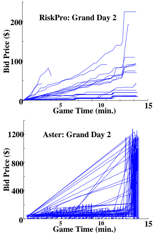
Figure 2: Graphs of two different agents’ bidding patterns over many games. Each line represents one game’s worth of bidding in a single auction. Above: RiskPro never bids over $250 in the games plotted. Below: Aster consistently bids over $1000 for rooms.
