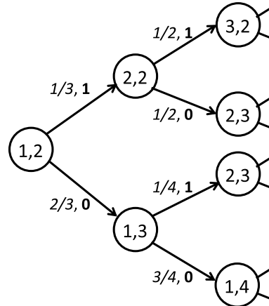
Figure 5: The Markov chain model for a Bayesian learning agent observing a sequence of \{0, 1\} values received for attending a sequence of hockey games. Each state is labeled with counts (N_1^t, N_0^t) of the number of value 1 and value 0 observations current period t . Transitions are labeled with a probability (depending on the relative counts) and the value received.
