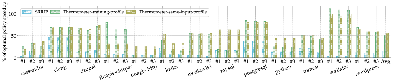
Figure 13: Thermometer 's IPC speedup across different application inputs as the percentage of the optimal BTB performance
