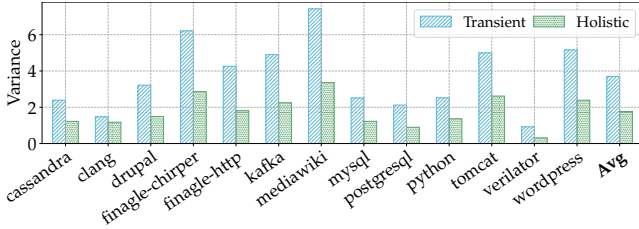
Figure 5: Average transient and holistic reuse distance variance for data center applications: the transient variance is significantly larger (more than 2×) than the holistic variance.
