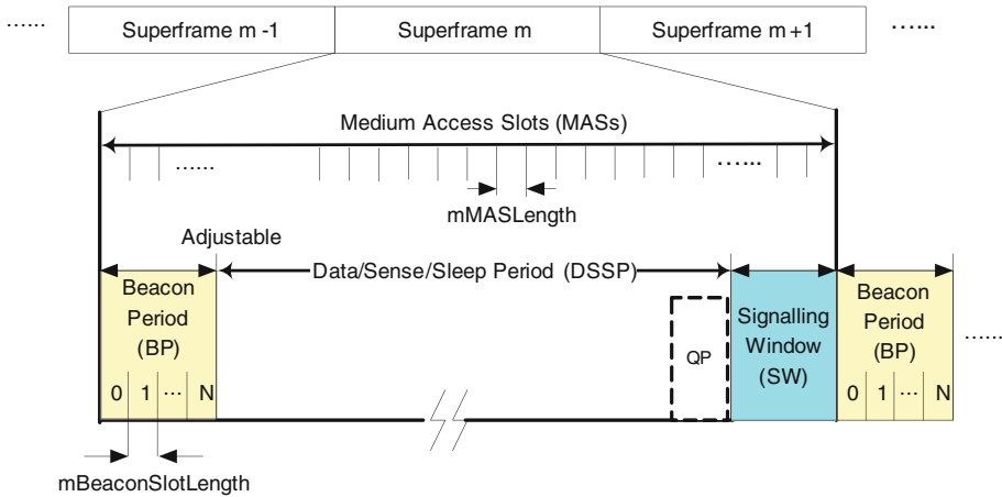
Fig. 2 QPDP MAC superframe structure
