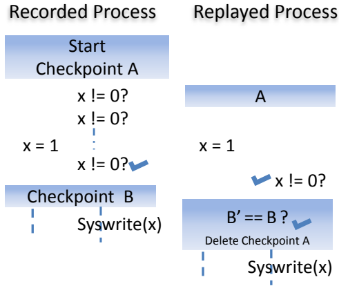
Figure 2.2: A data race that leads to convergent state
