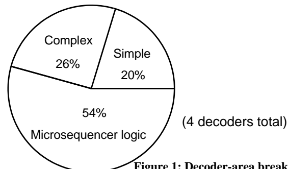
Figure 1: Decoder-area breakdown.
