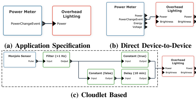
Fig. 12: Describing an application using a block editor. An application, shown in (a) and conceptually described as “when devices in a space are drawing power, turn on the lights”, is implemented in two ways using a block-connecting approach. In (b), the chosen power meter and lights have ports that match the description, allowing a direct connection to satisfy the specification. In (c), a different power meter (“Monjolo”) is used that sends pulses proportional to the metered load. The pulse stream must be filtered and fed into a type conversion block (“Constant”) to generate an “On” signal. A “Delay” block is used to automatically turn off the lights. As the dashed area generates “PowerChangeEvent”s, the application requirements are now satisfied. Because this application performs additional processing, it is run in a cloudlet. Implementing the same application description in multiple ways demonstrates how the architecture is able to adapt to changing devices.
