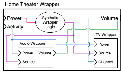
Fig. 4: Device wrapper for a synthetic “Home Theater” device. By including the wrappers for an audio device and a television with some additional logic, a home theater interface can be created without reimplementing the logic for communicating with the contained devices. This example demonstrates how a synthetic device can be created to provide a useful interface.
