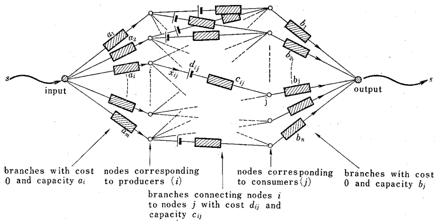
Fig. 2.4.1. Capacitated Hitchcock Problem
