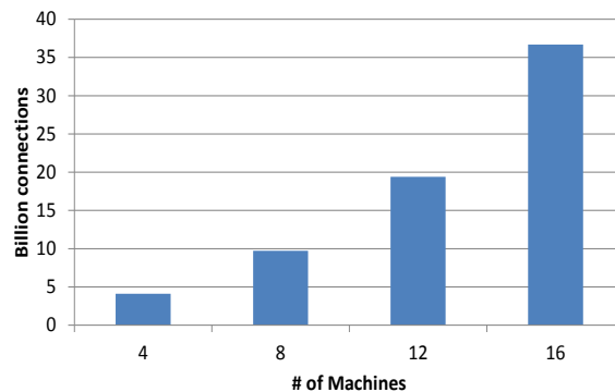
Figure 10. Scaling Model Size with more Workers.
