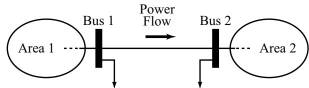
Fig. 1. Illustration of inappropriate undervoltage load shedding.
