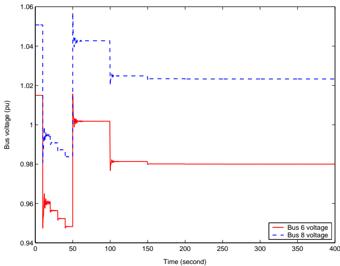
Fig. 9. Voltage response, imprecise load response.
