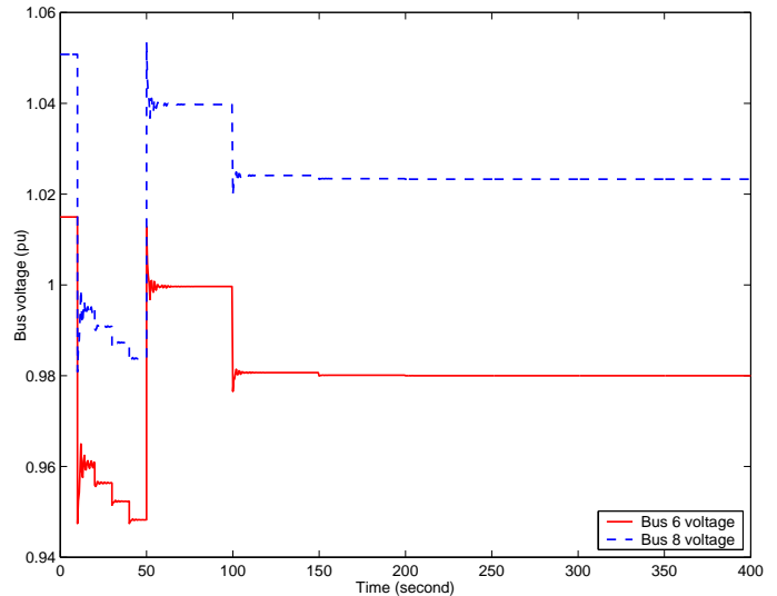
Fig. 7. Voltage response, perfect MPC model.
