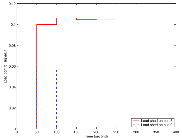
Fig. 8. Load control signals, perfect MPC model.
