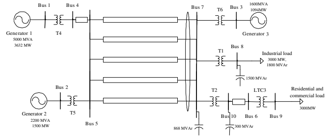
Fig. 4. Voltage collapse test system.
