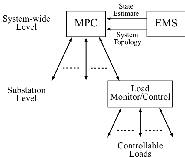
Fig. 2. Hierarchical load control structure.
