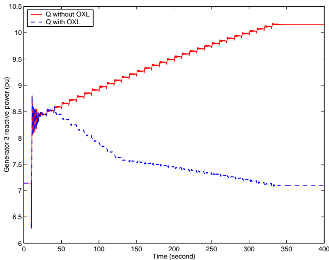
Fig. 6. Reactive support provided by generator 3, without MPC.
