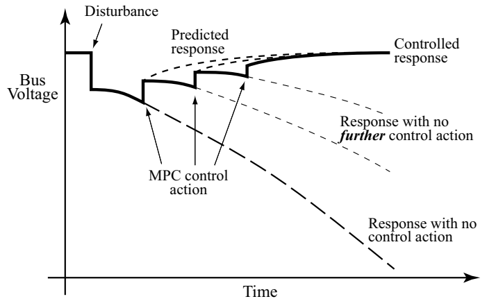
Fig. 3. MPC response.
