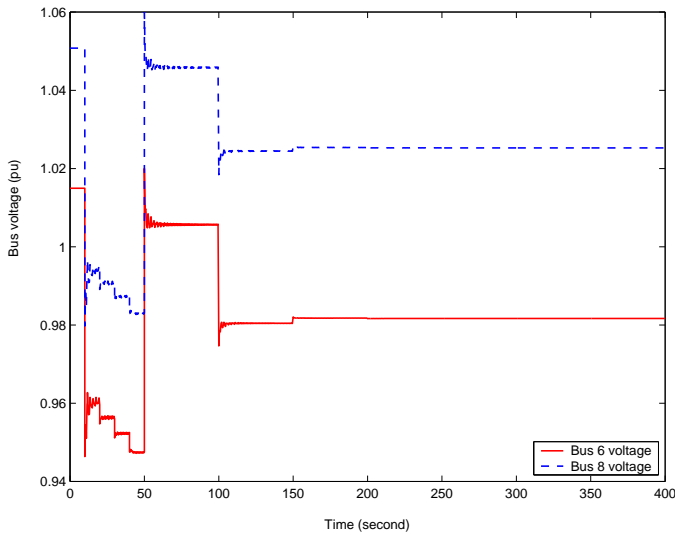
Fig. 10. Voltage response, realistic implementation.
