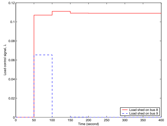
Fig. 11. Load control signals, realistic implementation.
