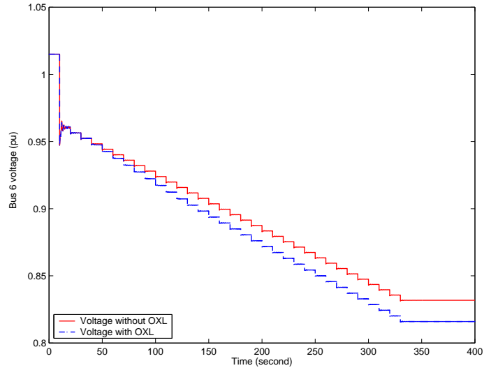
Fig. 5. Voltage response without MPC.
