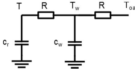
Figure 4. 2R-2C circuit model for the room thermal dynamics.
